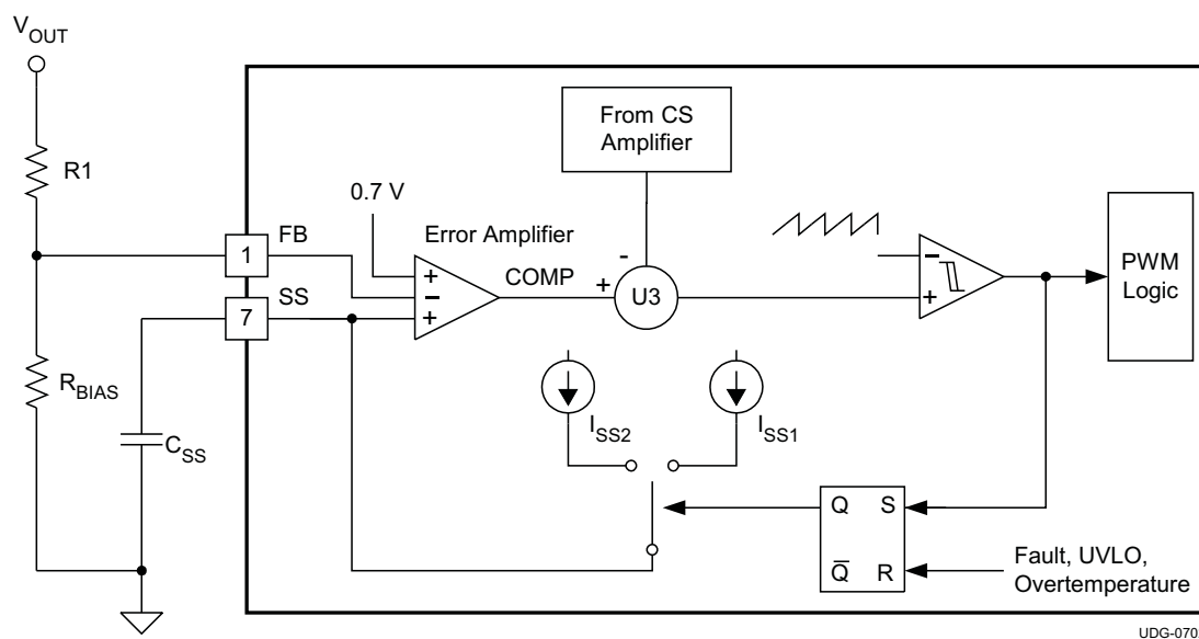
Figure 23. Soft-Start Implementation
