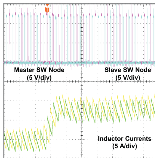
Figure 45. Current Balance at 0 A to 16 A Load Step Up, 2.5 A/μs Slew Rate
