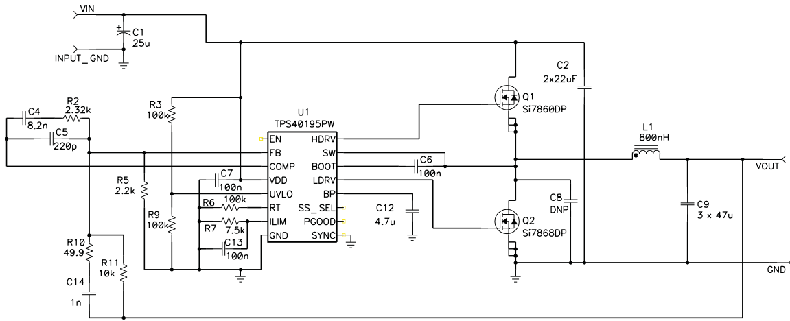
Figure 29. Design Example 2 Schematic
