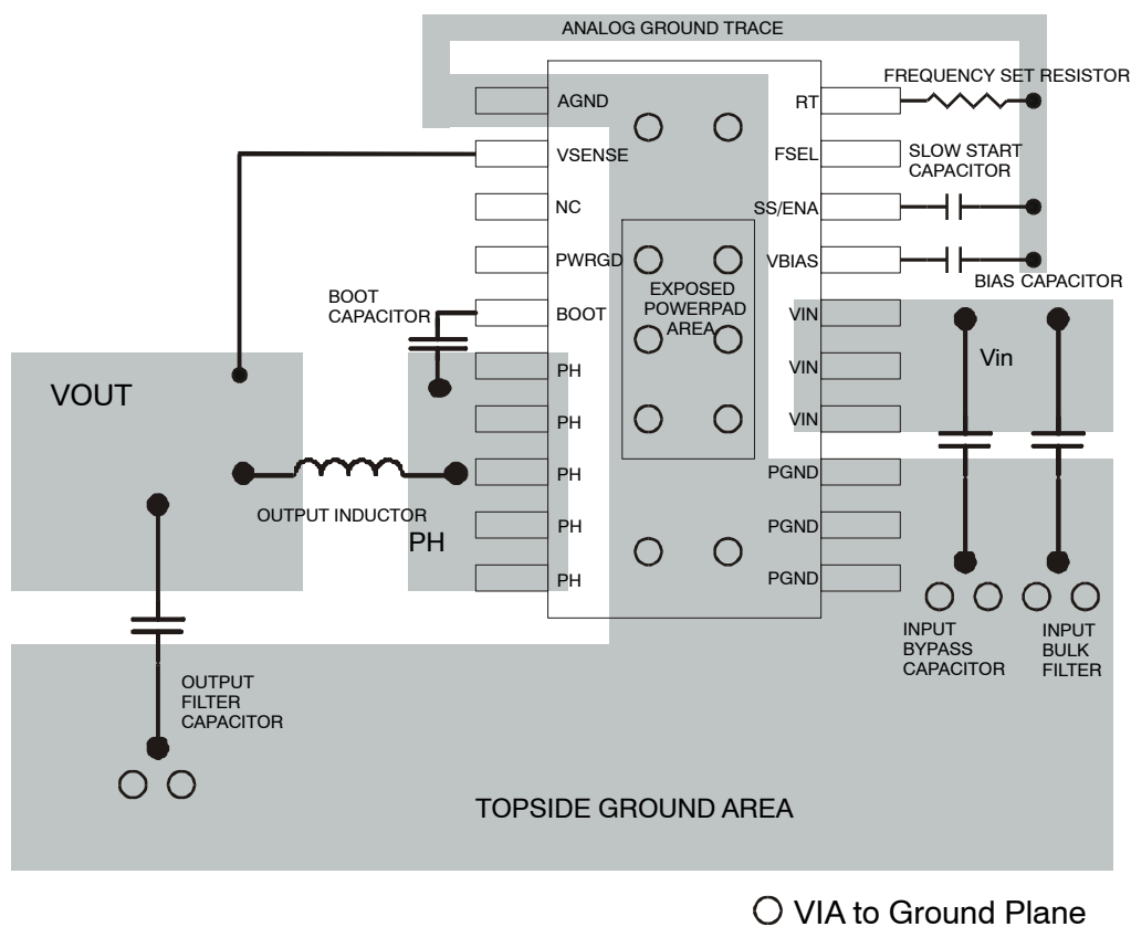
Figure 11. TPS54311 – 16 PCB Layout
