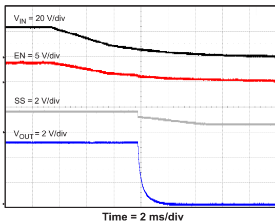
Figure 53. TPS54336 Shut Down Relative to VIN
