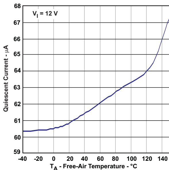
LPM, QUIESCENT CURRENT VARIATION WITH TEMPERATURE
