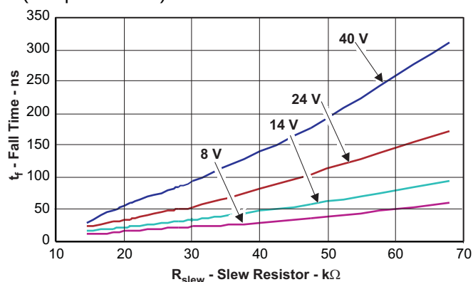
Figure 15. FET Fall Time
