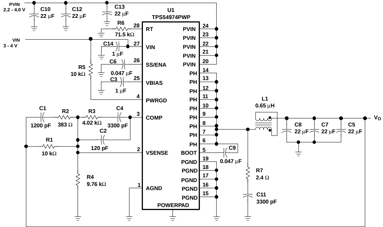
Figure 10. Application Circuit
