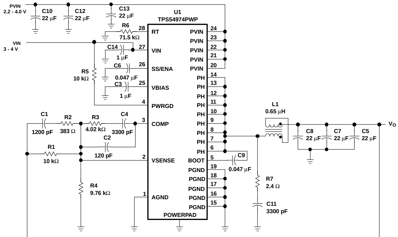
Figure 10. Application Circuit
