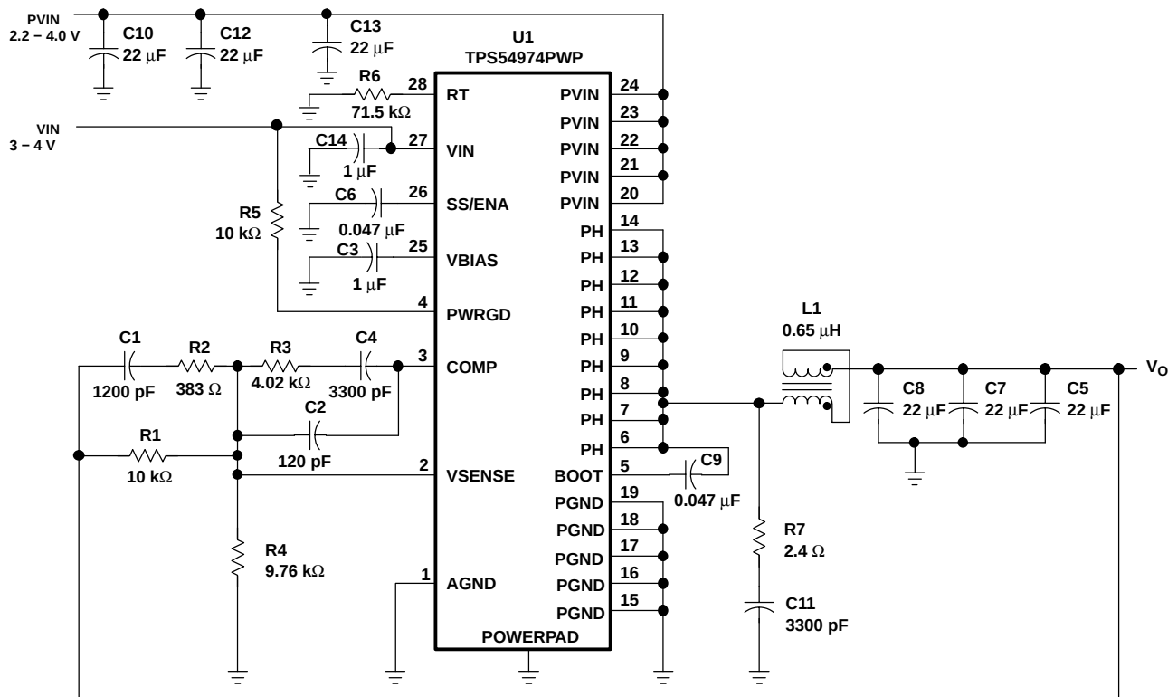
Figure 10. Application Circuit
