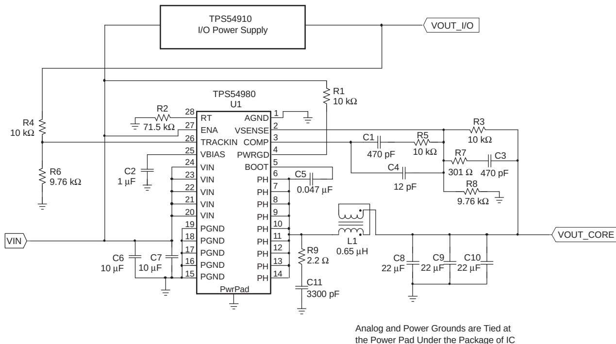
Figure 9. Application Circuit
