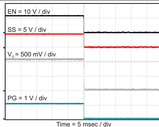
Figure 32. TPS562210 Shut Down Relative To EN
