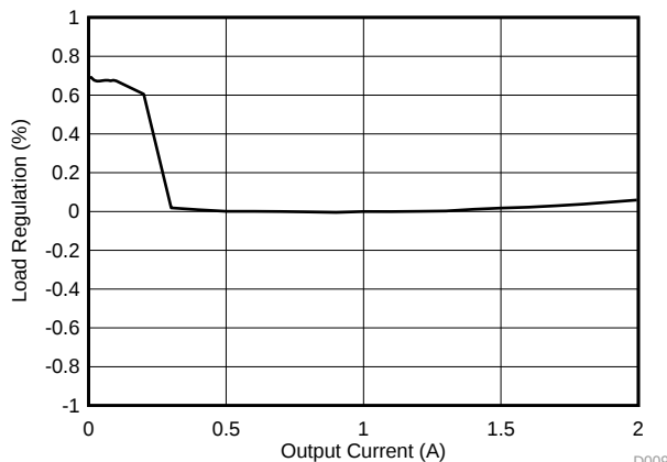
Figure 22. TPS562210 Load Regulation, V_I = 12\text{ V}
