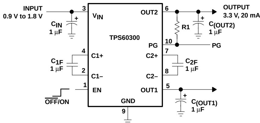
Figure 20. Typical Operating Circuit
