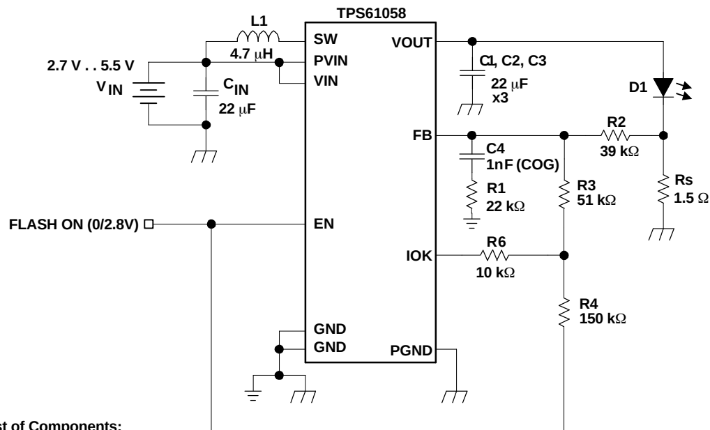
Figure 24. 500 mA Flashlight Application - 2.8 V Logic
