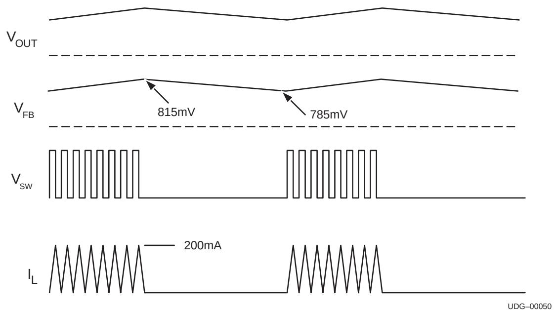
Figure 4. Typical Pulsed-Variable-Frequency Mode (PFM) Circuit Waveform
