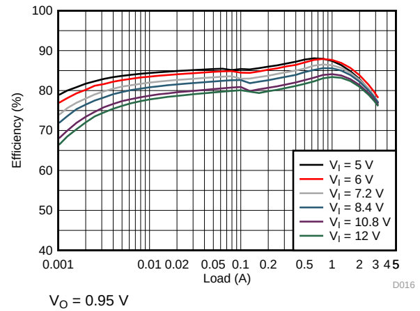
Figure 7. TPS62134B Efficiency
