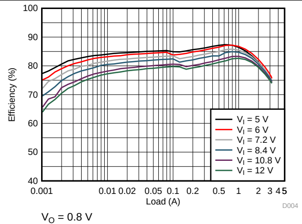
Figure 9. TPS62134C Efficiency
