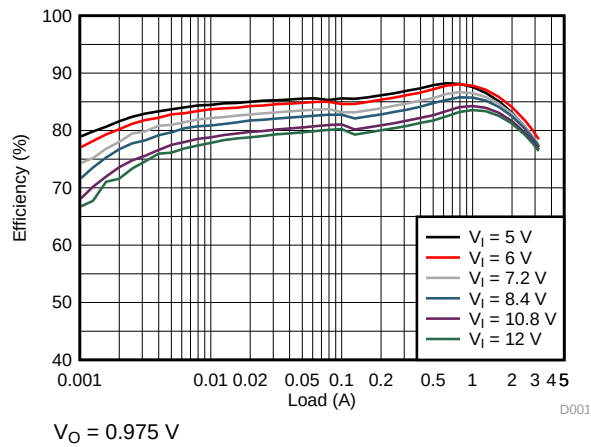
Figure 6. TPS62134A Efficiency
