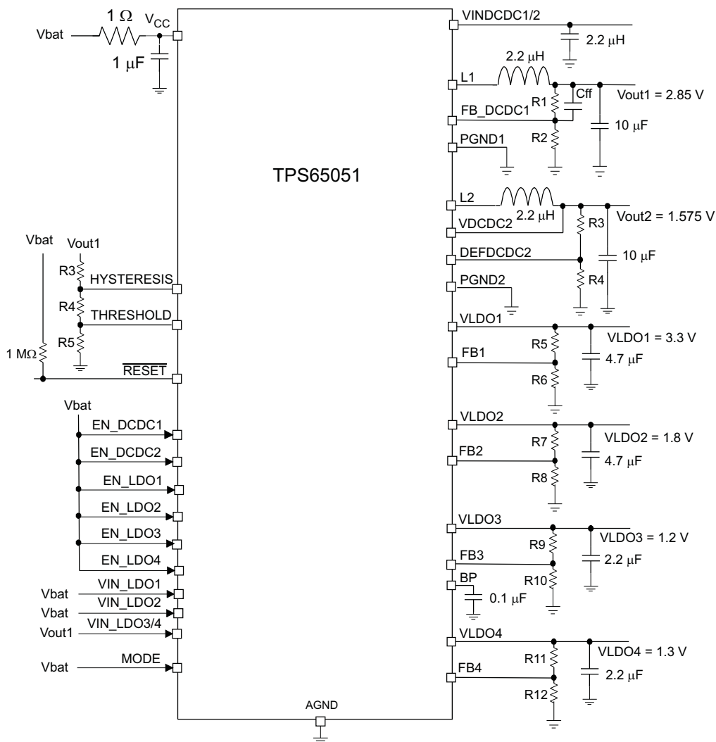
Figure 26. RESET Circuit
