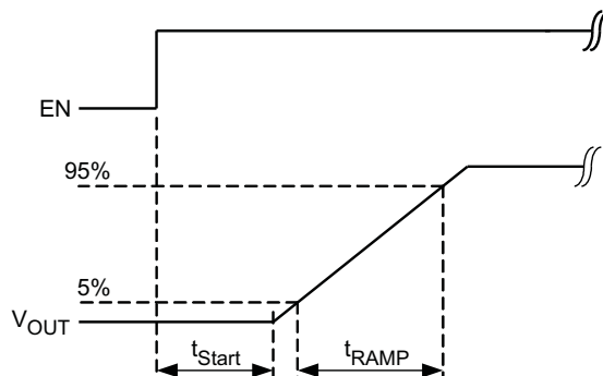
Figure 20. Soft Start
