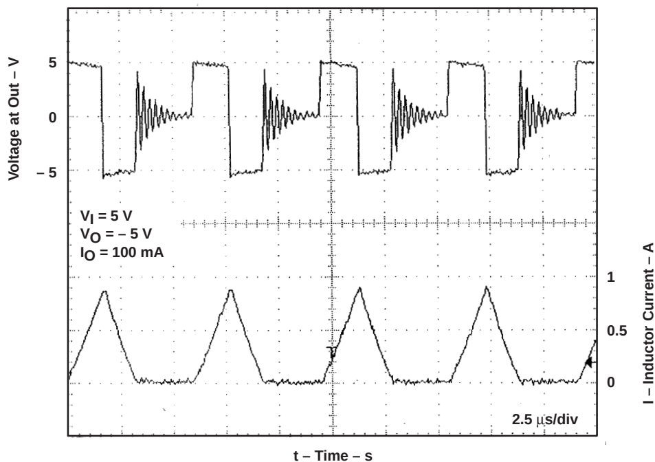
Figure 2. Switching Waveforms
