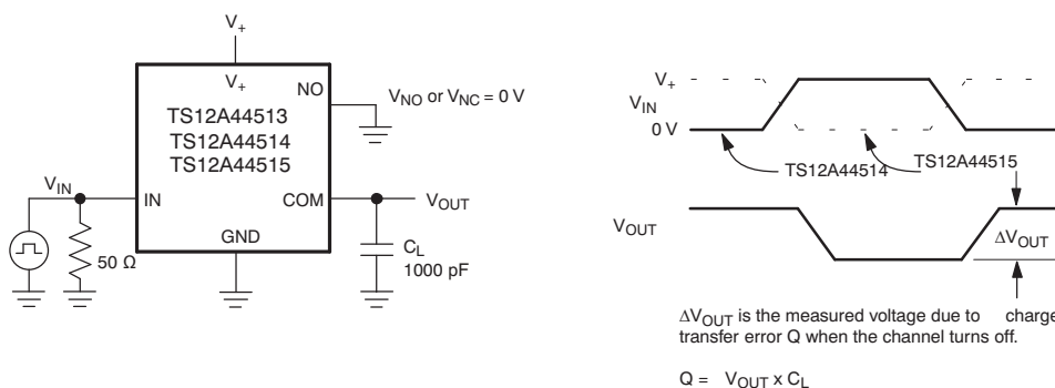
Figure 5. Charge Injection
