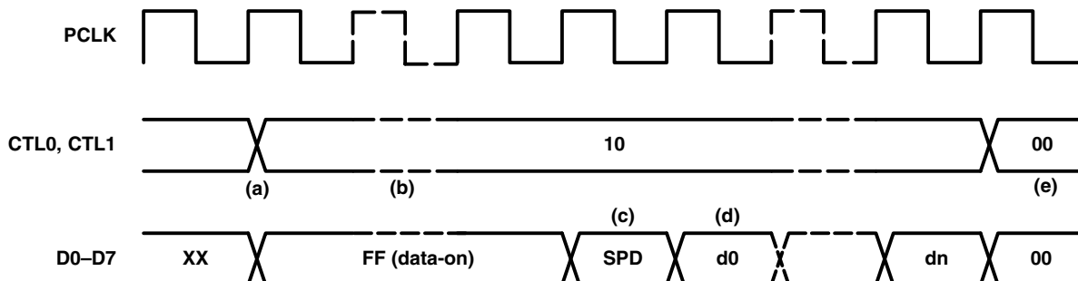
Figure 24. Normal Packet Reception Timing
