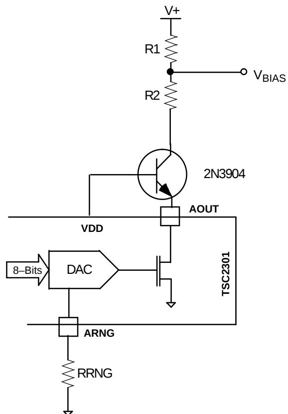
Figure 72. DAC Circuit When Using V+ Higher Than V_{\text{supply}} .
