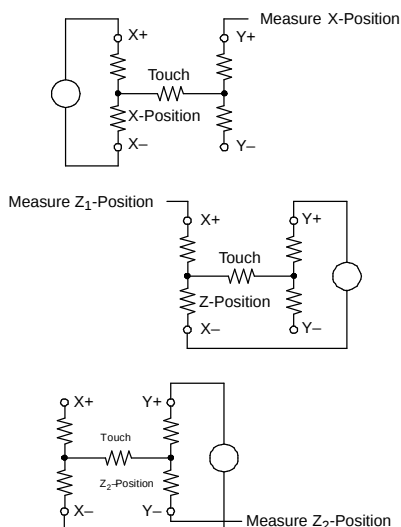
Figure 41. Pressure Measurement
