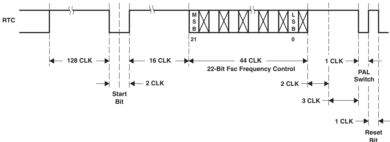
Figure 3-7. RTC Timing
