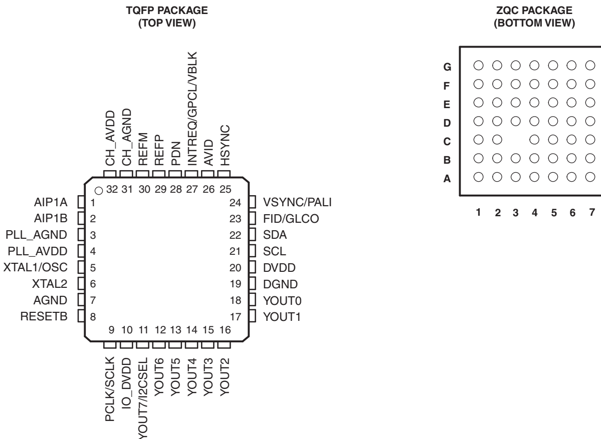
Figure 2-2. Terminal Diagrams
