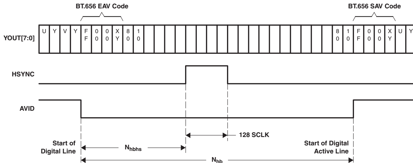
Figure 3-9. Horizontal Sync
