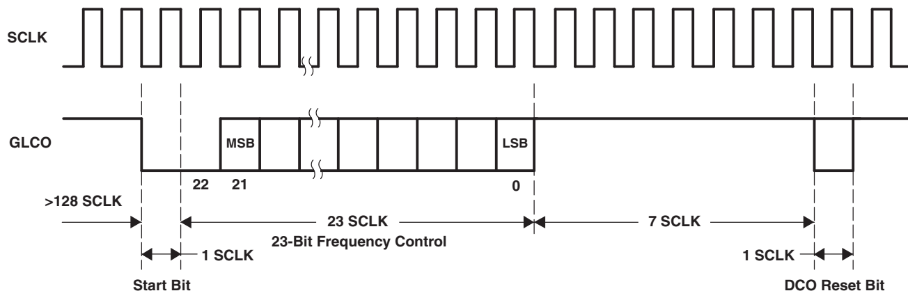
Figure 3-6. GLCO Timing
