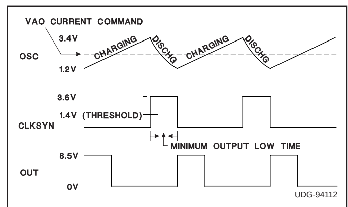
Figure 2. Oscillator and PWM Output Waveform
