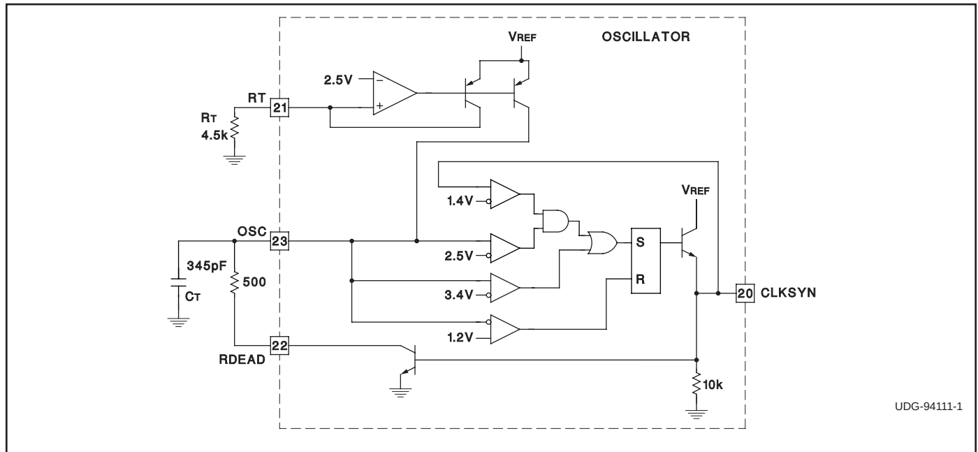
Figure 1. Oscillator Block with External Connections
