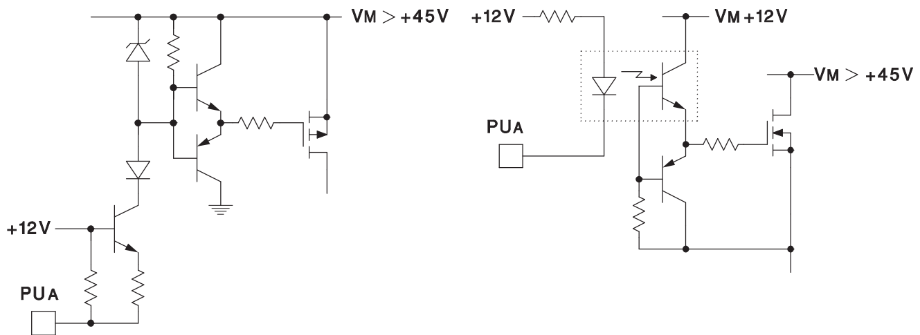
Figure 9. Fast High-Side P-Channel Driver
