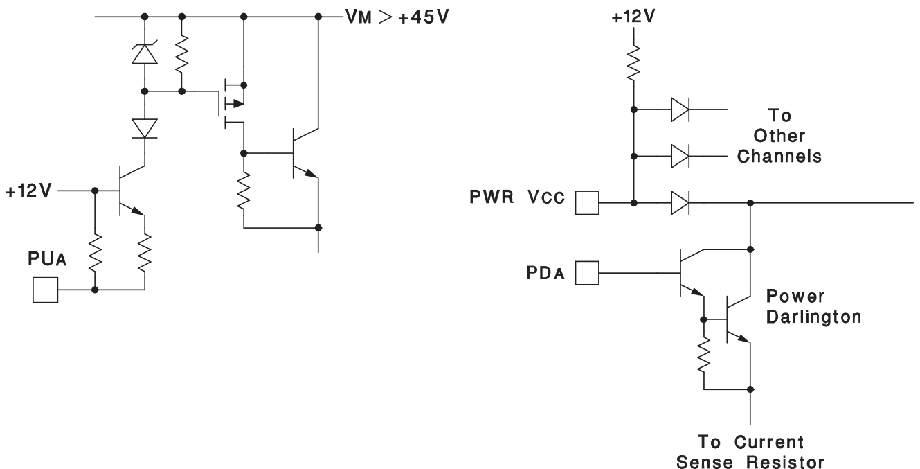
Figure 11. Power NPN High-Side Driver
