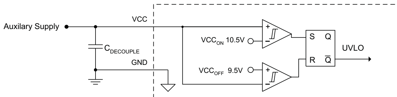
Figure 22. UVLO
