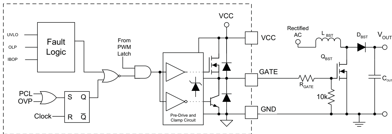
Figure 26. Gate Driver
