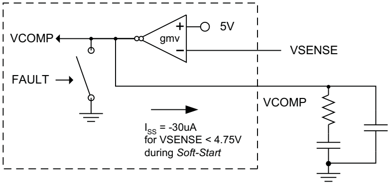
Figure 20. Soft Start
