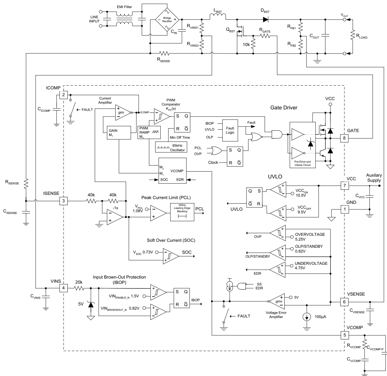
Figure 18. Block Diagram
