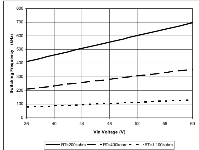
Figure 32. Switching Frequency Variation Over the Input Voltage for Fixed Volt-Second Mode of Operation
