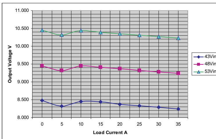
Figure 57. Load regulation
