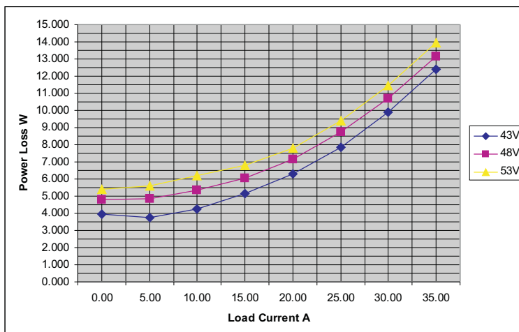
Figure 56. . Power Dissipation
