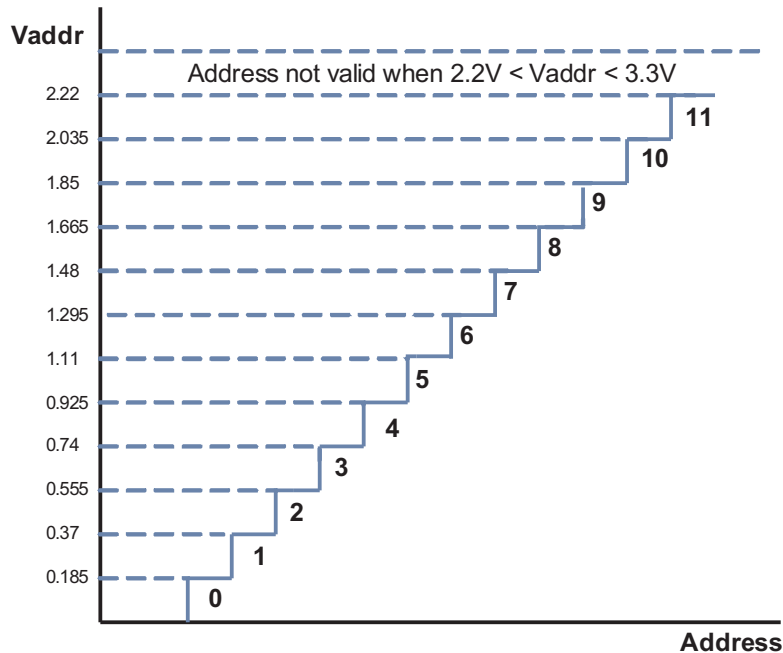
Figure 5. V ADDR to PMBus Address Translation
