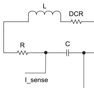
Figure 7. Inductor Current Sensing Circuit
