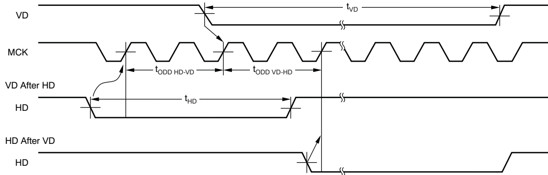
Figure 2. VD, HD Falling Edge Detect
