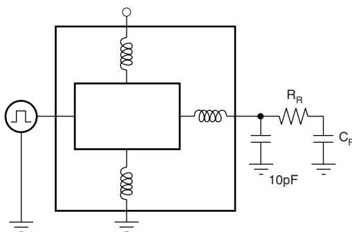
Figure 11. RG Driver and Load Model
