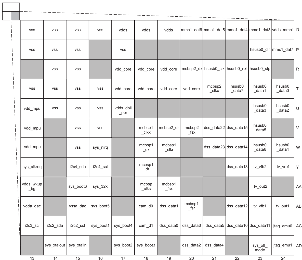
Figure 2-17. CUS Pin Map [Quadrant D - Top View]
