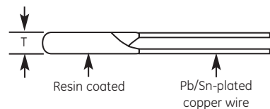
Power thermistor standard dimensions
