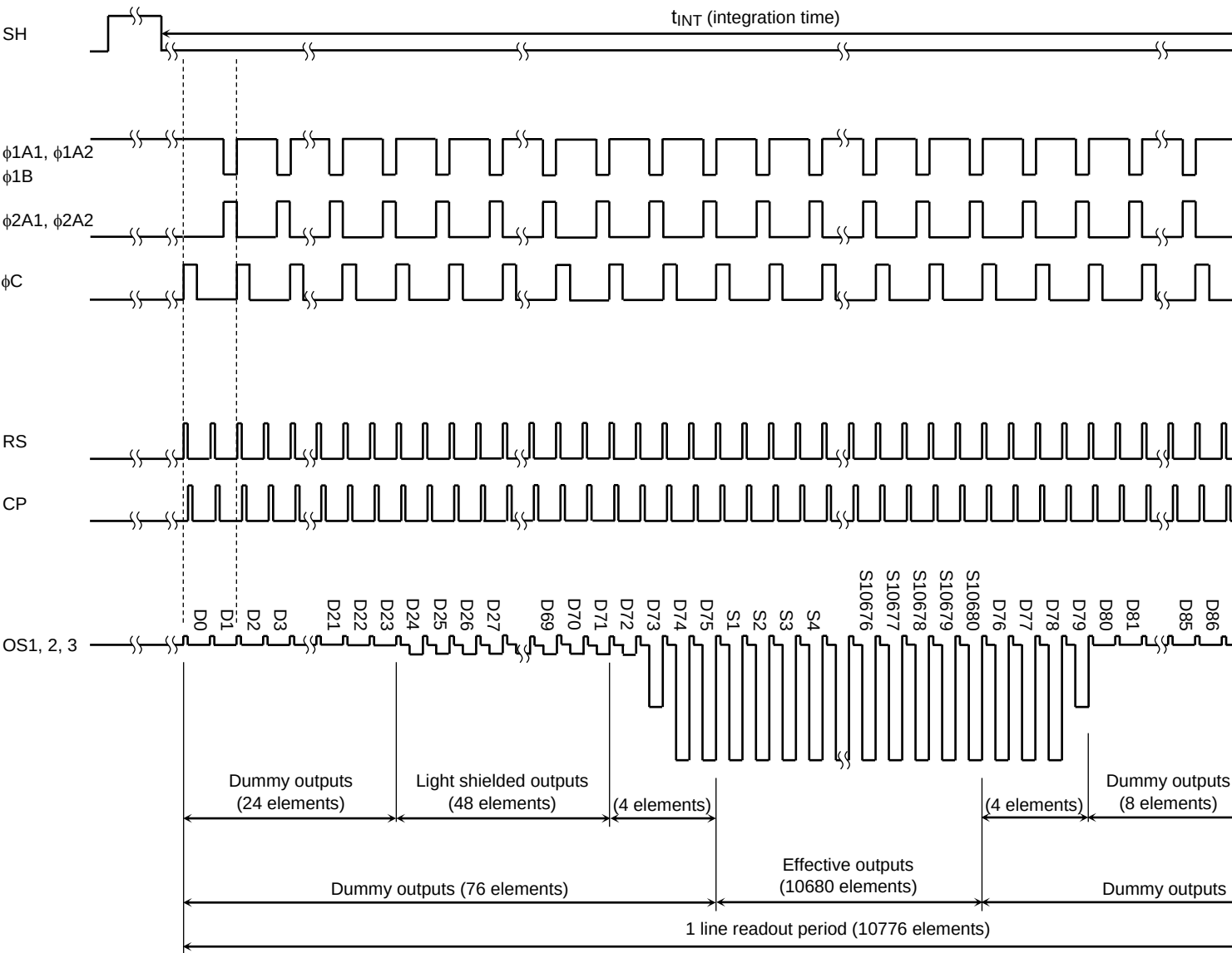
Timing Chart 1: 1200 dpi Mode (Bit Clamp Mode)
