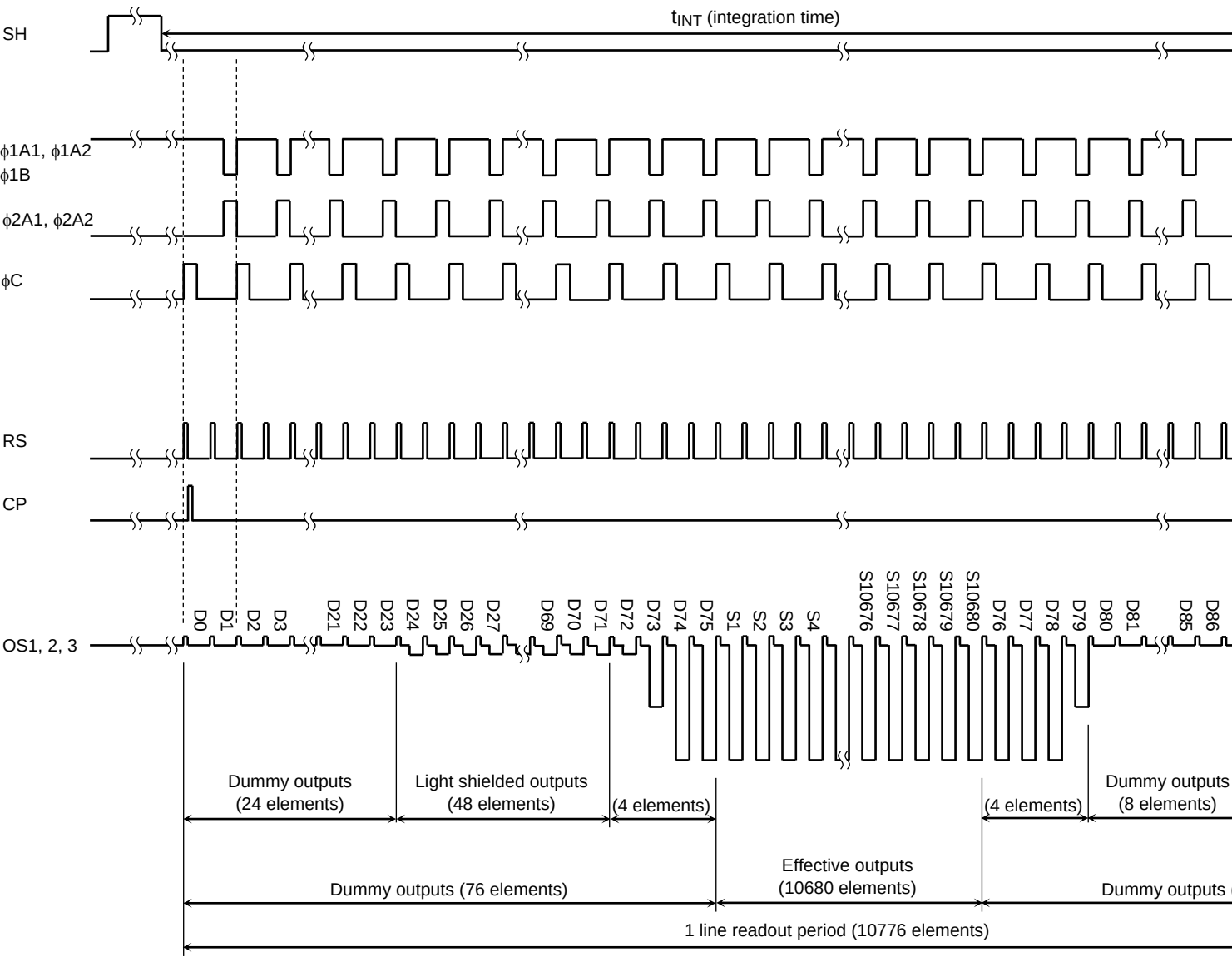
Timing Chart 2: 1200 dpi Mode (Line Clamp Mode)
