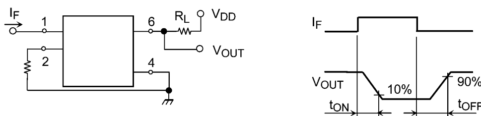
Fig. 12.1 Switching Time Test Circuit and Waveform
