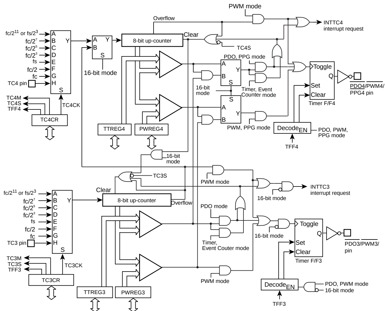
Figure 9-1 8-Bit TimerCounter 3, 4
