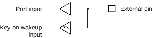
Figure 13-2 Key-on Wakeup Input and Port Input
