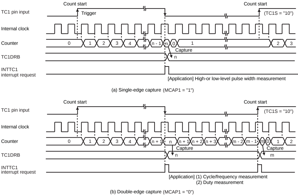
Figure 8-6 Pulse Width Measurement Mode
