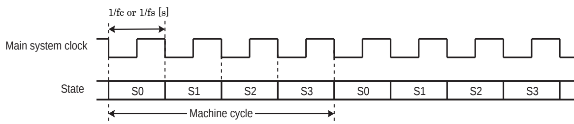
Figure 2-5 Machine Cycle
