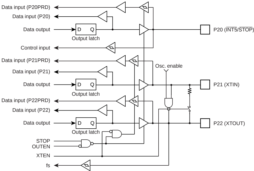
Figure 7-4 Port 2
