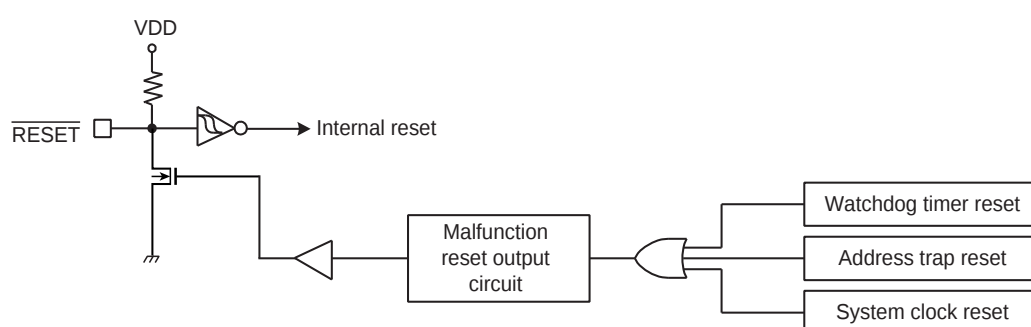
Figure 2-15 Reset Circuit
