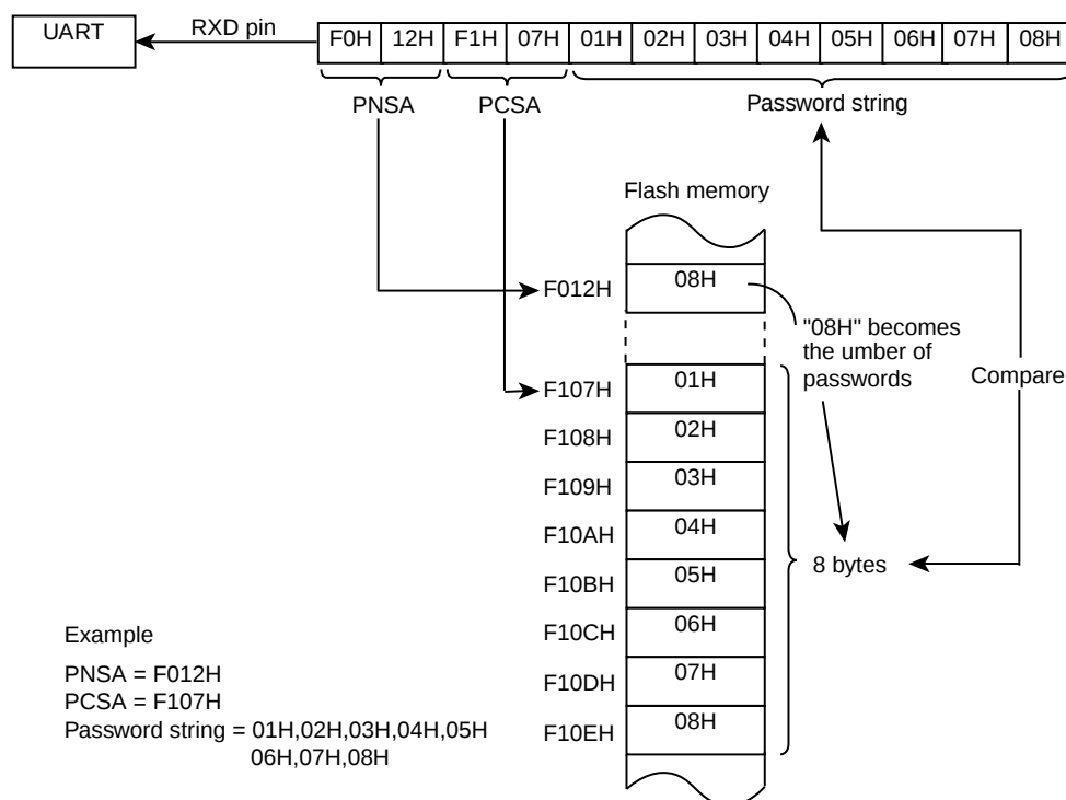
Figure 15-5 Password Comparison
