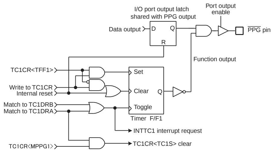
Figure 8-7 PPG Output
