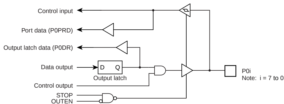
Figure 7-2 Port 0
