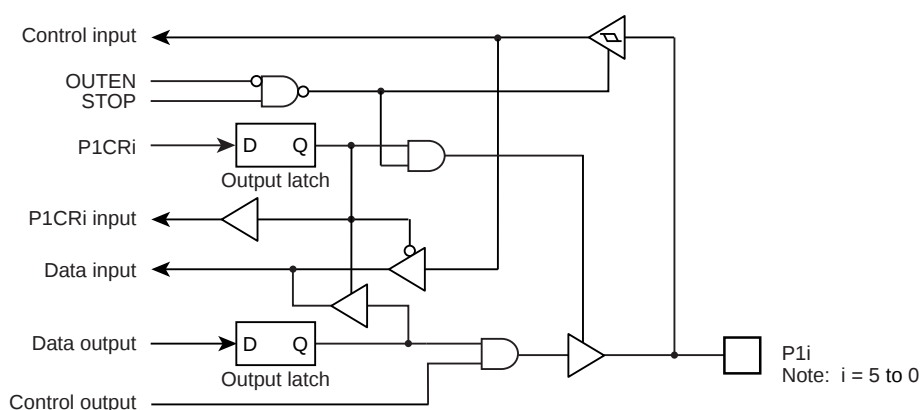
Figure 7-3 Port P1
