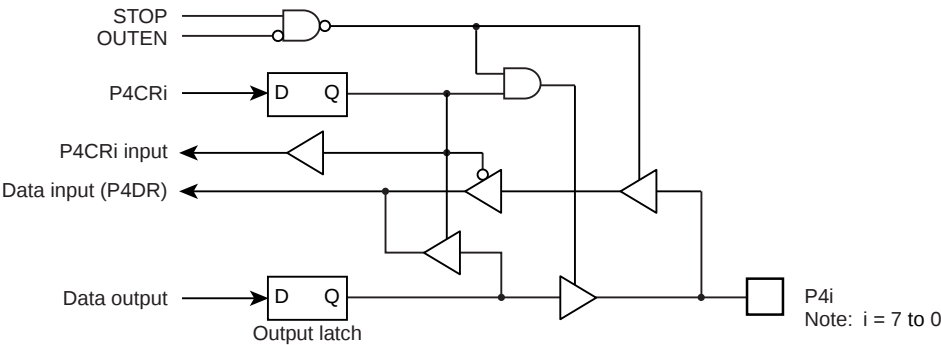
Figure 7-6 Port P4
