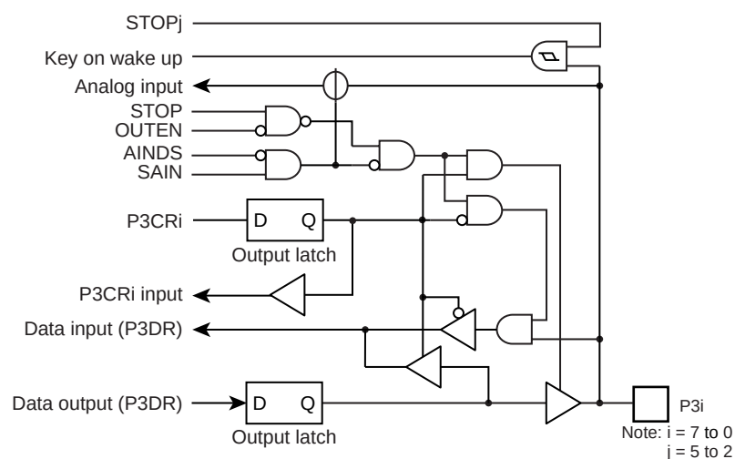
Figure 7-5 Port P3
