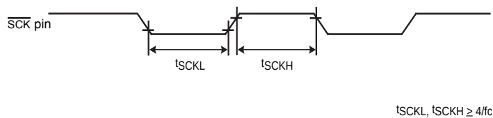
Figure 10-3 External Clock
