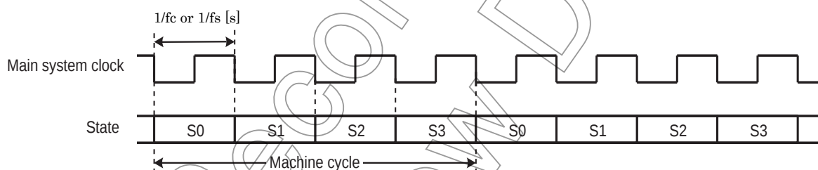
Figure 2-5 Machine Cycle
