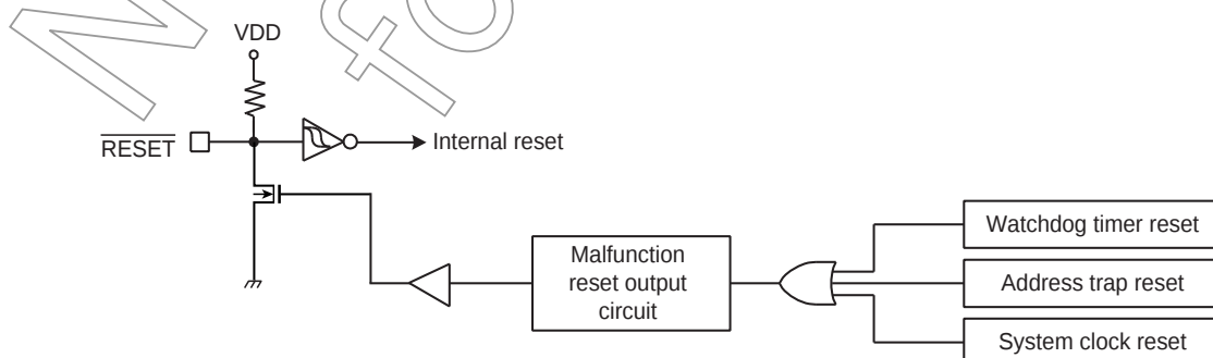
Figure 2-15 Reset Circuit
