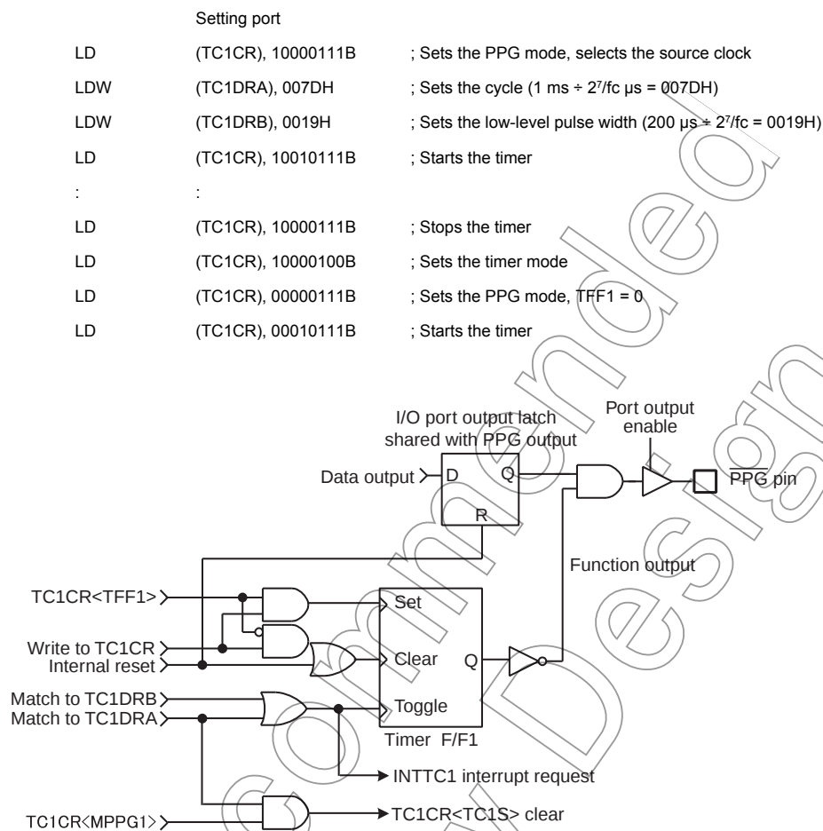
Figure 8-7 PPG Output
