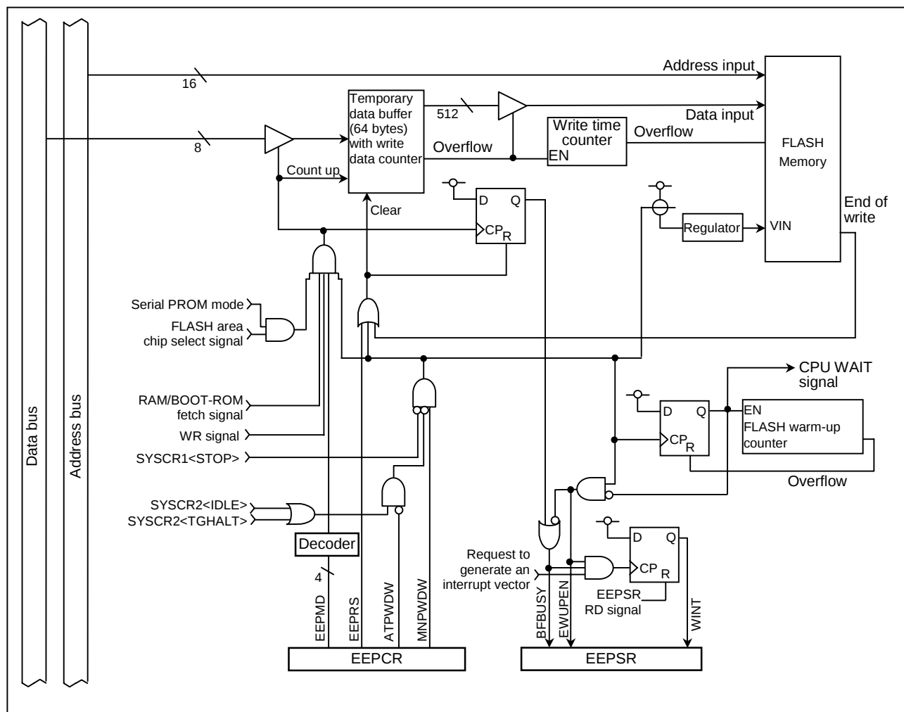
Figure 1.2.1 FLASH Memory Control
