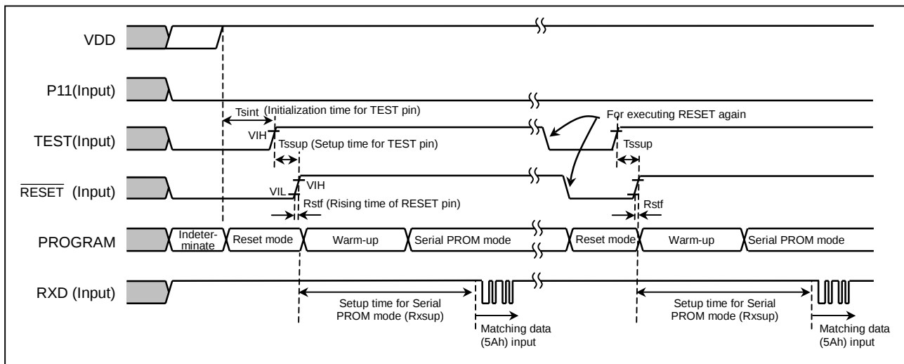
Figure 2.1.3 Serial PROM Mode Timing
