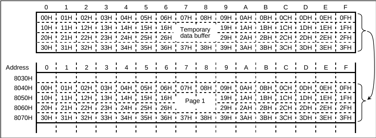
Figure 1.2.7 Data Buffer and Write Page (Example)
