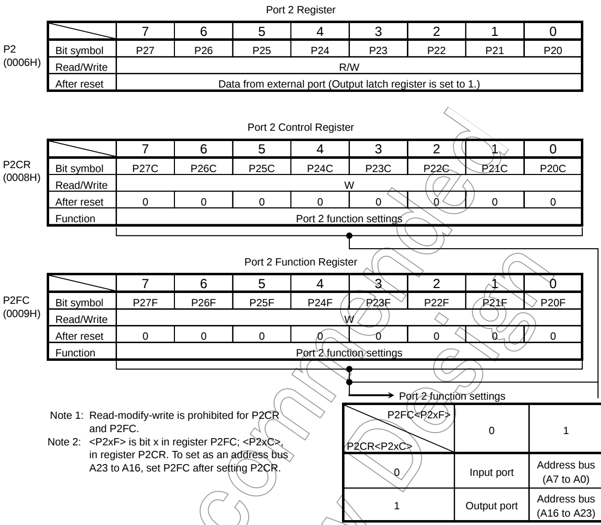
Figure 3.5.7 Register for Port 2
