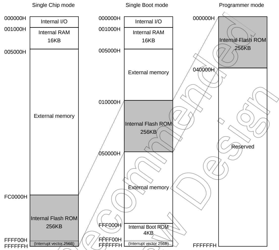
Figure 3.14.3 TMP91FY42 Memory Map for Each Operation Mode
