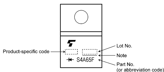
Fig. 7.2 Marking (Package Name: TOSHIBA 2-10AB1A)
