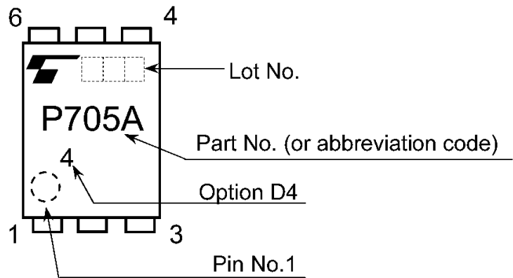
Fig. 16.4 Marking Example (Note)
