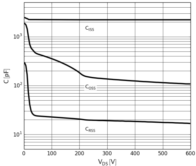
Figure 5. Typical Capacitance
