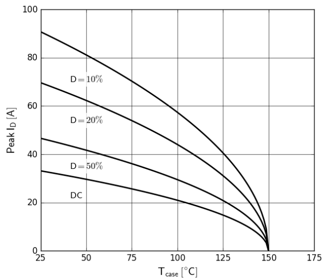
Figure 8. Current Derating
