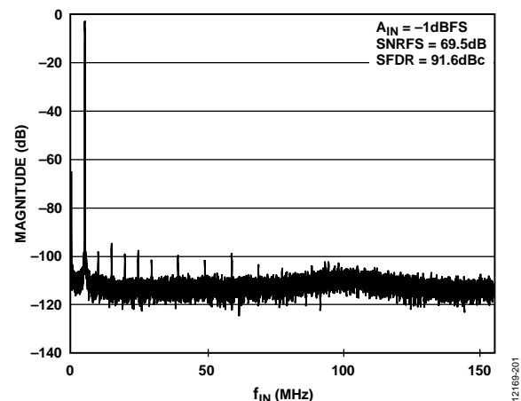
Figure 16. FFT f_{IN} = 305 MHz, A_{IN} = -1 dBFS, Dither On, Register 0x22A = 0x01
