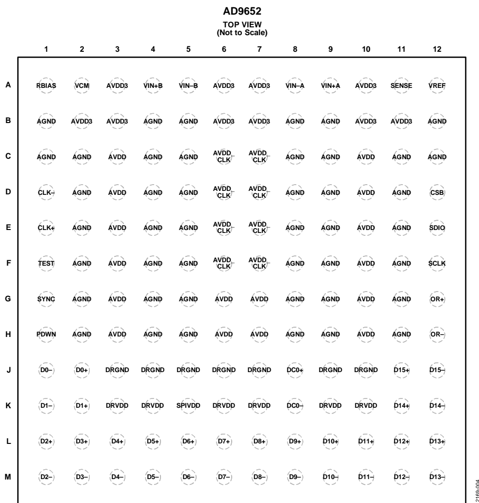
Figure 5. Pin Configuration
