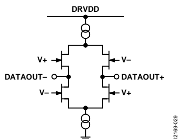
Figure 44. Equivalent LVDS Output Circuit (DCO±, OR±, and D0± to D15±)
