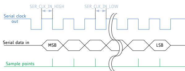
Figure 64: SSI: SSI_IN_CLK_DELAY =0
