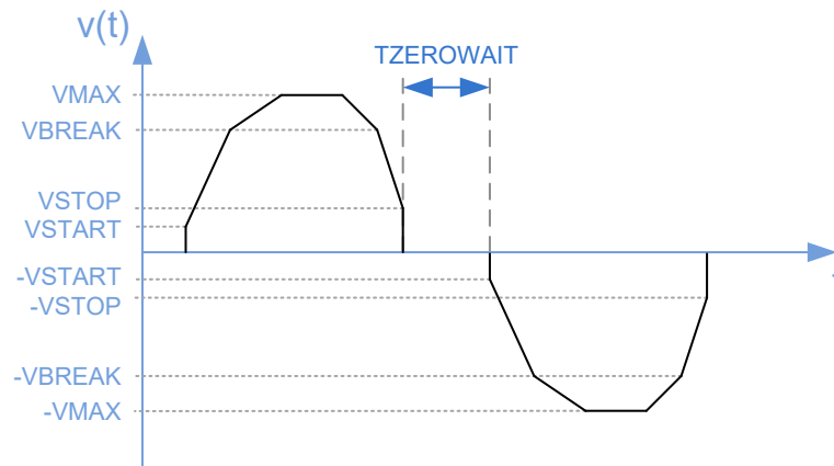
Figure 30: Example for U-Turn Behavior of sixPoint Ramp
