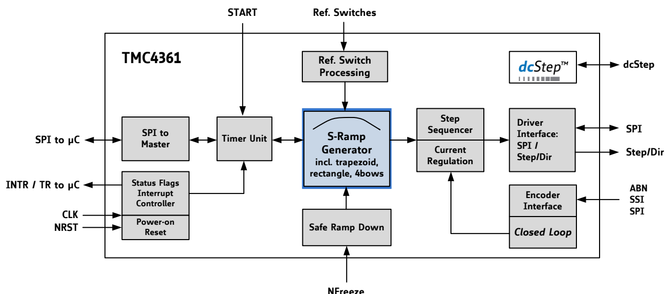
Figure 2: Block Diagram
