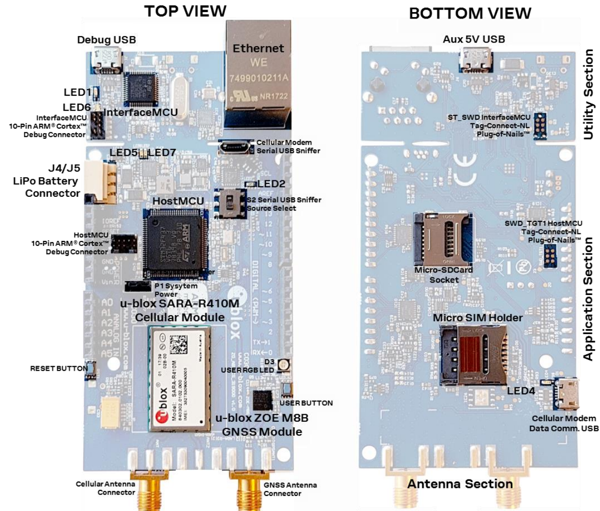
Figure 10: C030-R410M major component locations
