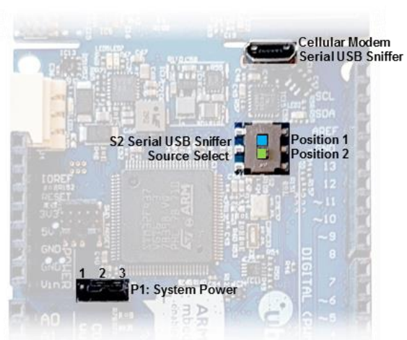
Figure 13: C030-R410M / C030-R3121 jumper and switches
