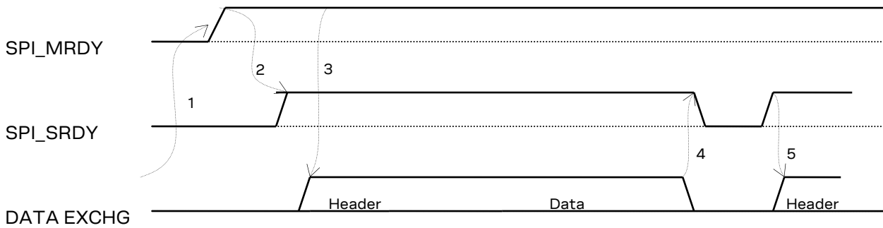
Figure 43: Data transfer initiated by the application processor (master) with a sleeping LISA-U2 module (slave)
