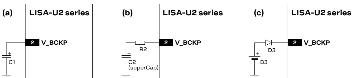
Figure 16: Real time clock supply (V_BCKP) application circuits: (a) using a 100 µF capacitor to let the RTC run for ~50 s after VCC removal; (b) using a 70 mF capacitor to let RTC run for ~10 hours after VCC removal; (c) using a non-rechargeable battery
