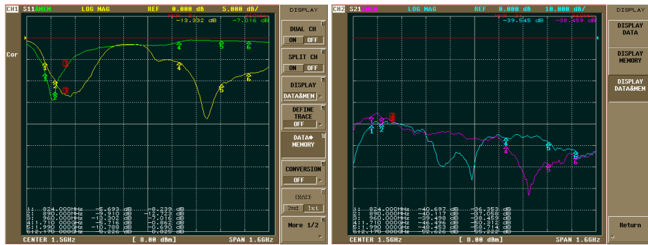
Figure 65: |S_{11}| and |S_{21}| comparison between a 900 MHz tuned half wavelength dipole (green/purple) and a penta-band internal antenna (yellow/cyan)
