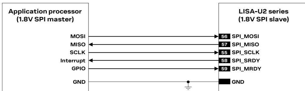
Figure 45: IPC / SPI Interface application circuit connecting LISA-U2 series 1.8V SPI slave to a 1.8V SPI master
