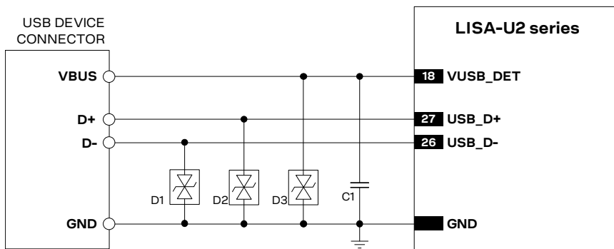
Figure 40: USB Interface application circuit
