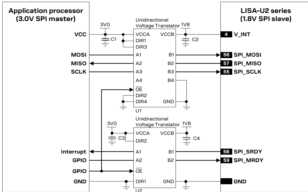
Figure 46: IPC / SPI Interface application circuit connecting LISA-U2 series 1.8V SPI slave to a 3.0 V SPI master
