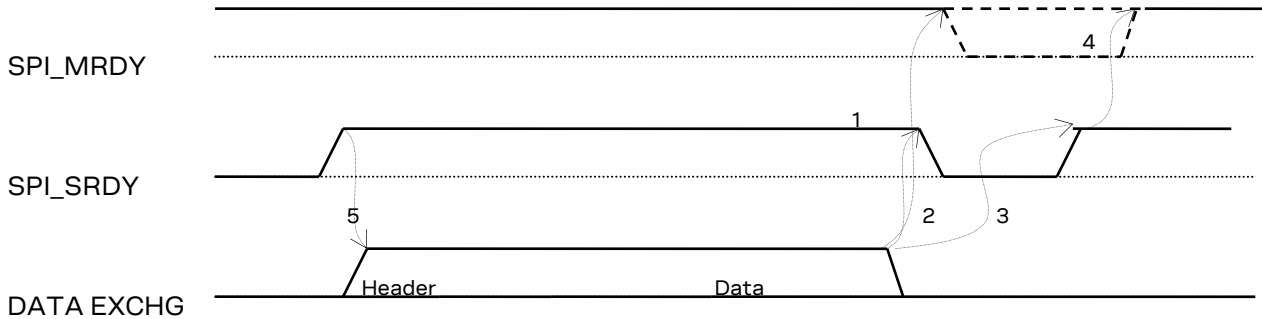
Figure 44: Data transfer terminated and then restarted by LISA-U2 module (slave)
