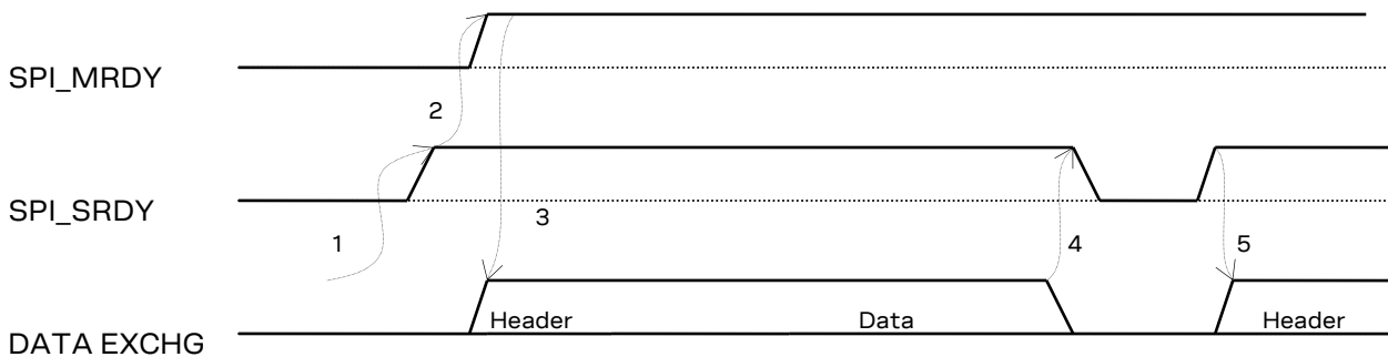
Figure 42: Data transfer initiated by the LISA-U2 module (slave), with a sleeping application processor (master)
