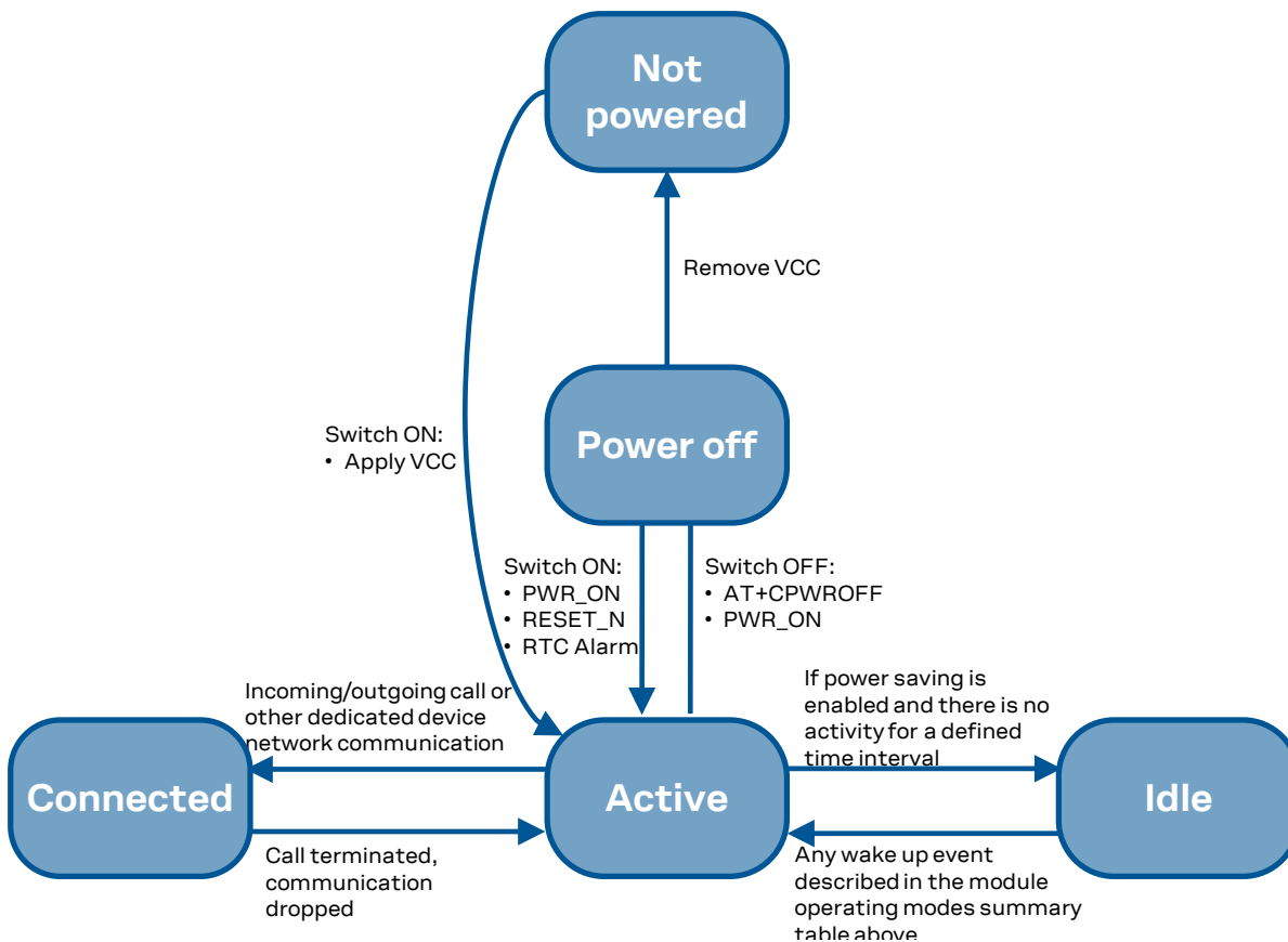
Figure 2: Operating modes transition
