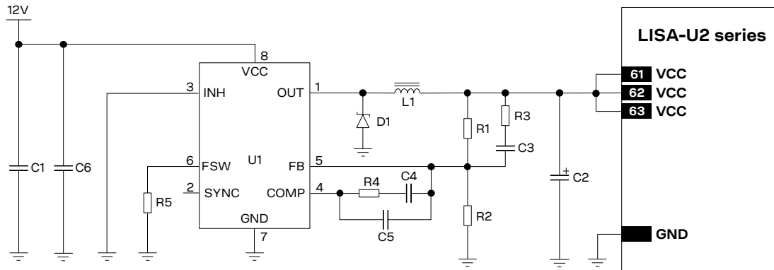
Figure 7: Suggested low cost solution for the VCC voltage supply application circuit using a step-down regulator
