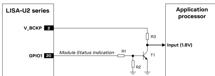
Figure 53: Module status indication application circuit
