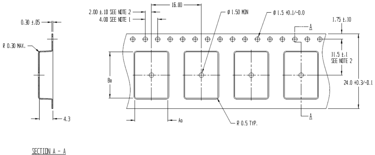
Figure 9: NINA-B221 tape dimension
