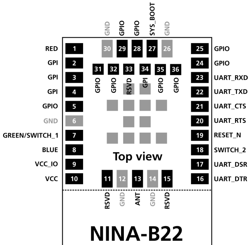
Figure 2: NINA-B22x pin assignment (top view)
