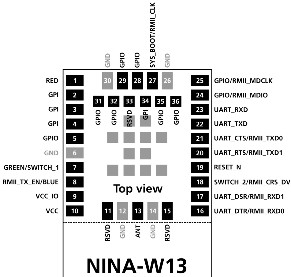
Figure 2: NINA-W13x pin assignment (top view)
