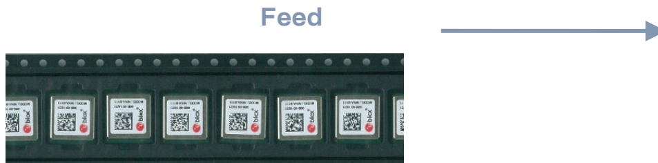
Figure 7: Orientation of NINA-W131 module on tape
