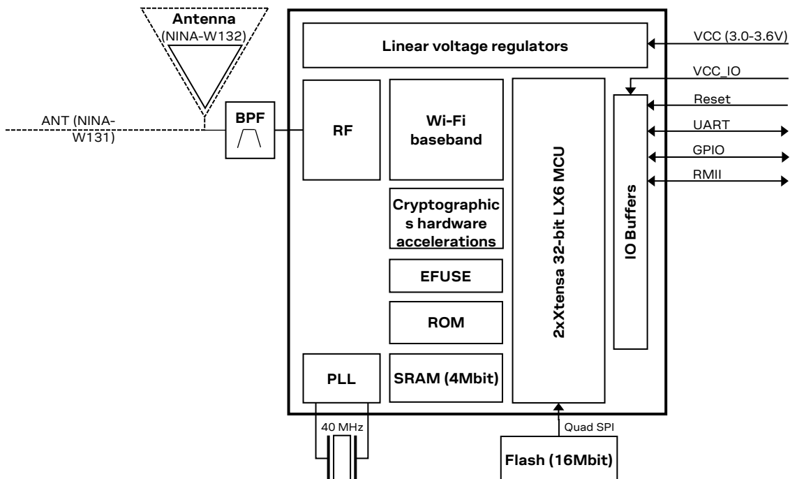
Figure 1: Block diagram of NINA-W13 series
