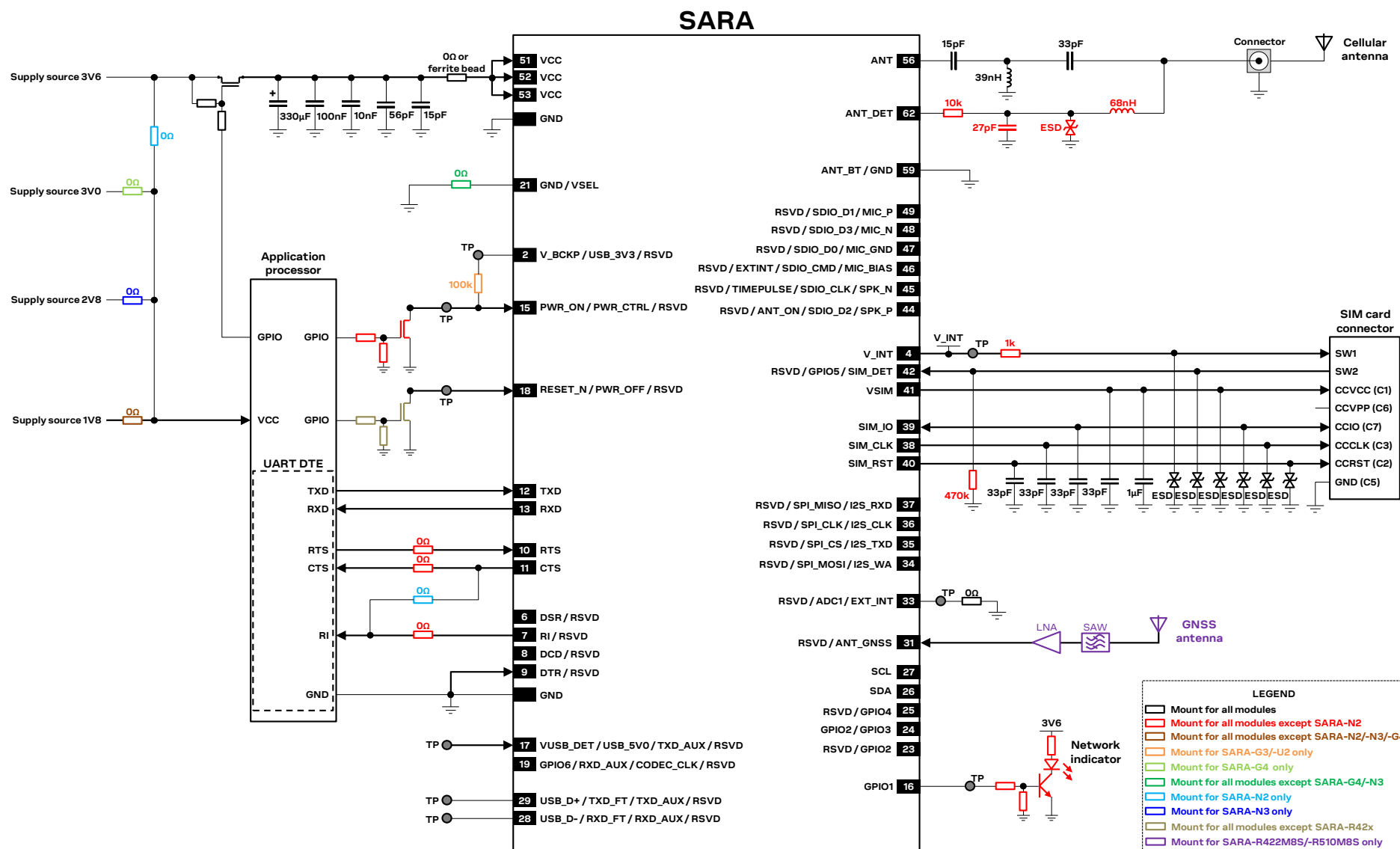
Figure 78: Example schematic to integrate a SARA-R4, SARA-R5, SARA-N2, SARA-N3, SARA-G3, SARA-G4 and/or SARA-U2 module in the same application PCB, using main interfaces
