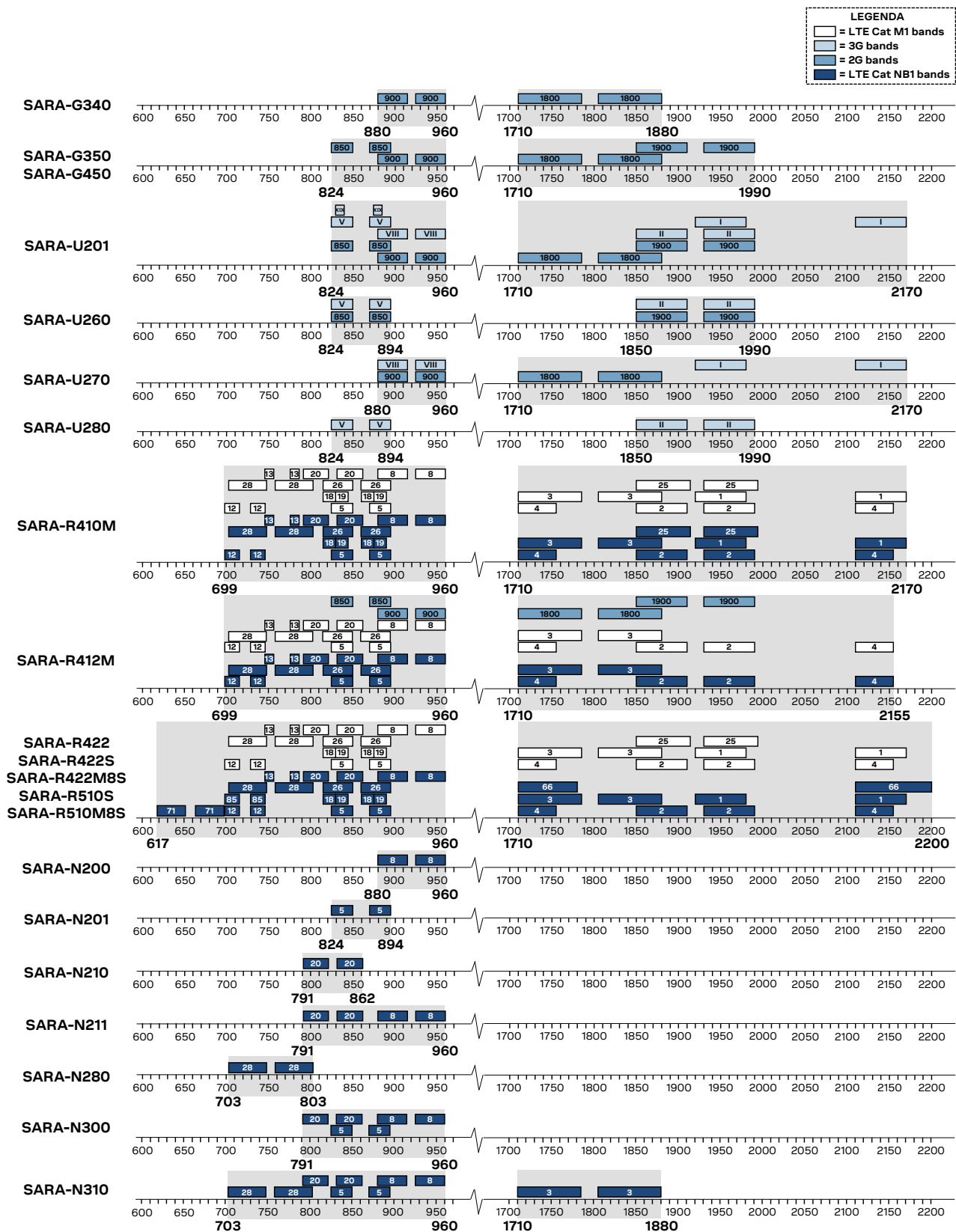
Figure 77: Summary of operating frequency bands supported by SARA modules
