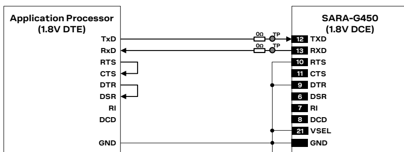
Figure 56: UART application circuit with partial V.24 link (3-wire) in the DTE/DCE serial interface (1.8 V DTE / 1.8 V DCE)
