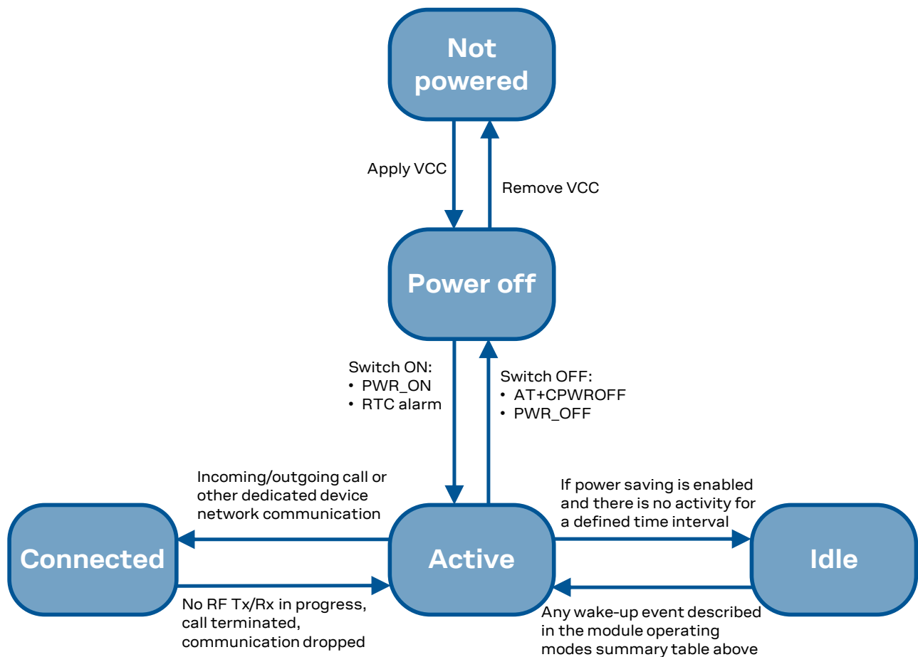
Figure 2: Operating modes transitions
