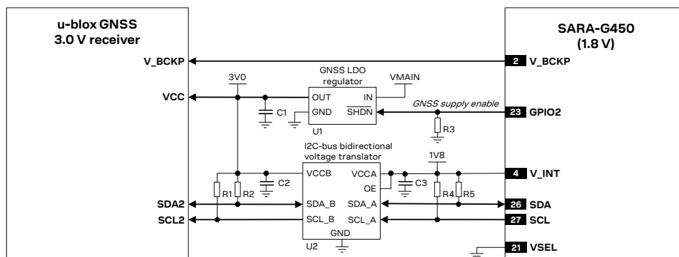
Figure 68: Application circuit for connecting SARA-G450 (1.8 V) modules to u-blox 3.0 V GNSS receivers
