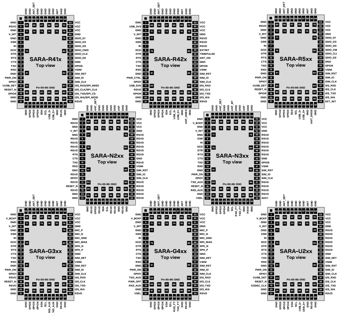
Figure 75: SARA-R4, SARA-R5, SARA-N2, SARA-N3, SARA-G3, SARA-G4, and SARA-U2 modules' layout and pin assignment
