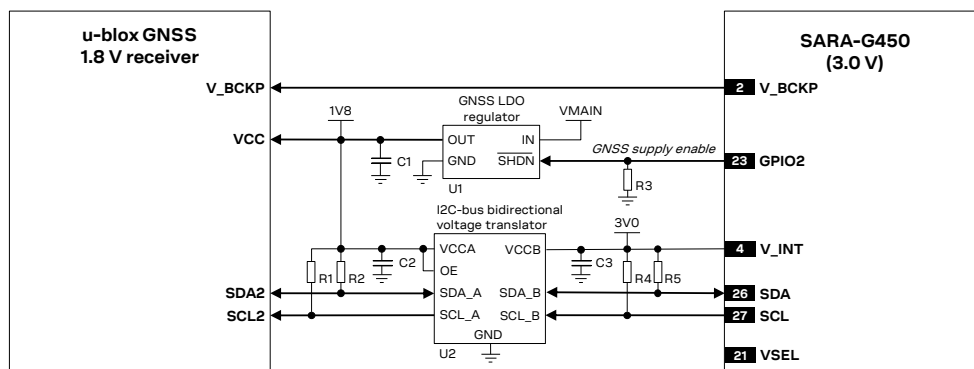
Figure 65: Application circuit for connecting SARA-G450 (3.0 V) modules to u-blox 1.8 V GNSS receivers
