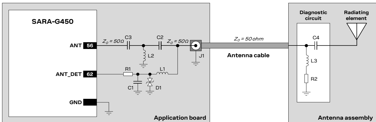
Figure 41: Suggested schematic for antenna detection circuit on application PCB and diagnostic circuit on antenna assembly
