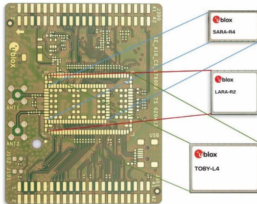
Figure 76: Cellular modules' layout compatibility: all modules can be mounted on the same nested footprint
