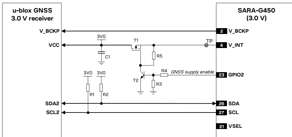
Figure 67: Application circuit for connecting SARA-G450 (3.0 V) modules to u-blox 3.0 V GNSS receivers using V_INT as supply
