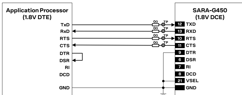
Figure 53: UART application circuit with partial V.24 link (5-wire) in the DTE/DCE serial interface (1.8 V DTE / 1.8 V DCE)
