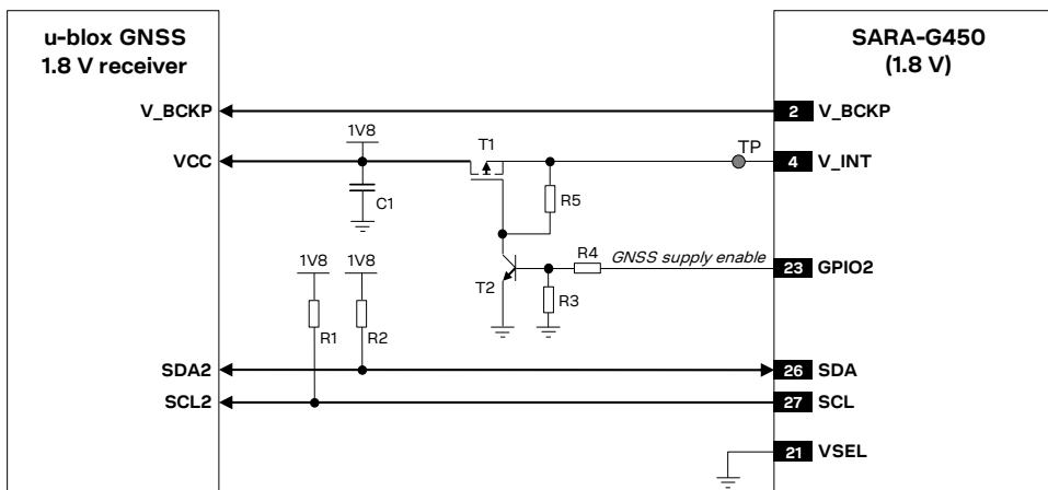
Figure 64: Application circuit for connecting SARA-G450 (1.8 V) modules to u-blox 1.8 V GNSS receivers using V_INT as supply
