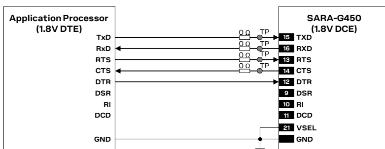
Figure 50: UART application circuit with partial V.24 link (6-wire) in the DTE/DCE serial communication (1.8 V DTE / 1.8 V DCE)
