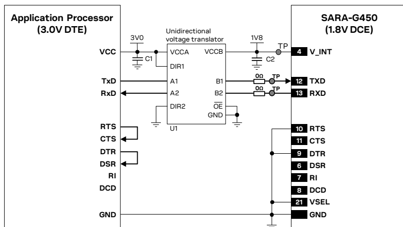
Figure 58: UART application circuit with partial V.24 link (3-wire) in the DTE/DCE serial interface (3.0 V DTE / 1.8 V DCE)
