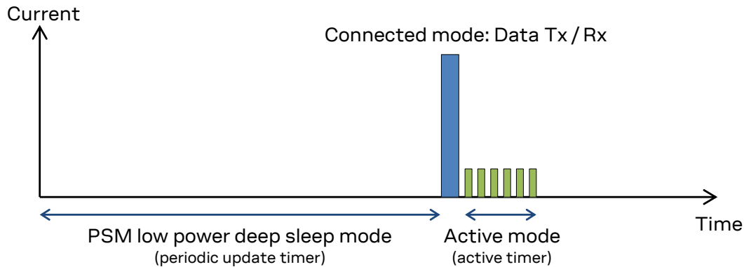
Figure 14: Description of the PSM timing
