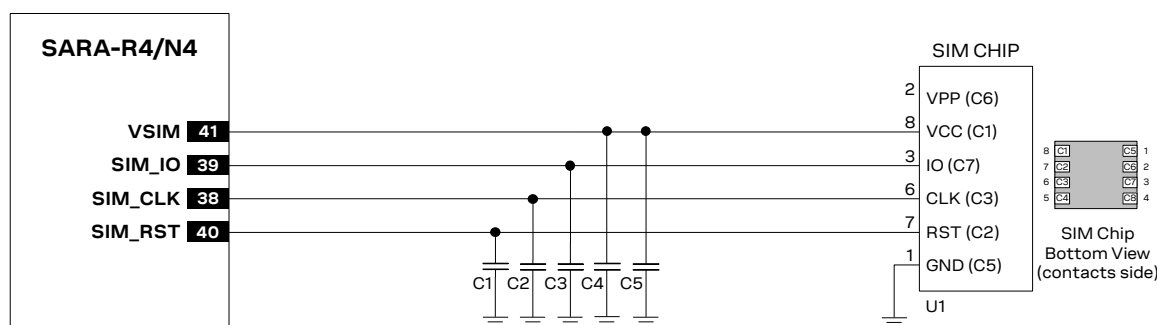
Figure 38: Application circuits for the connection to a single Surface-Mounted SIM chip, with SIM detection not implemented
