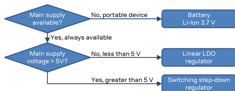
Figure 15: VCC supply concept selection
