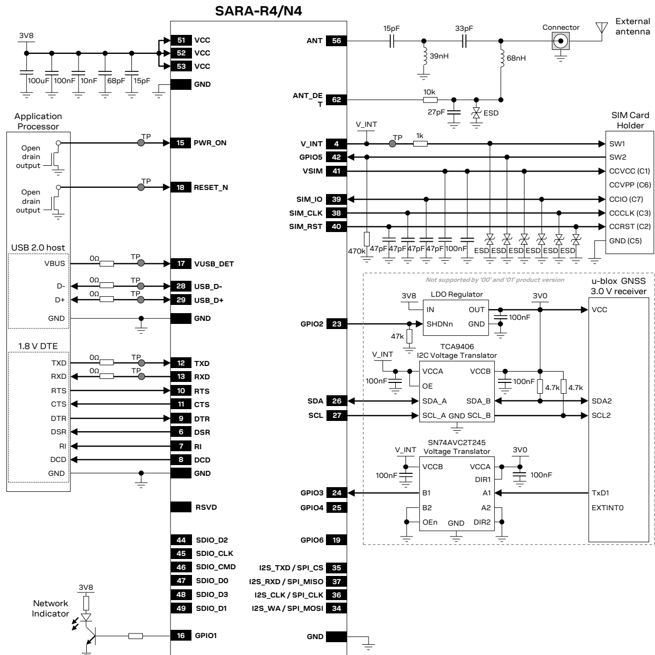
Figure 55: Example of schematic diagram to integrate a SARA-R4 series module using all available interfaces 25
