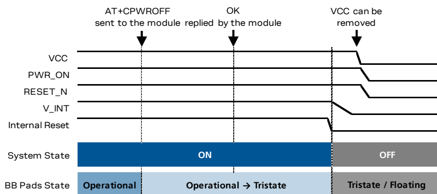
Figure 10: SARA-R4 series modules switch-off sequence by means of AT+CPWROFF command
