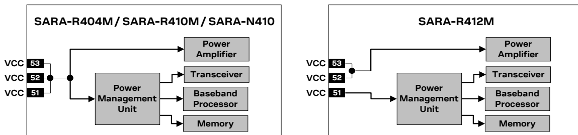
Figure 3: Block diagram of SARA-R4 series modules' internal VCC supply routing
