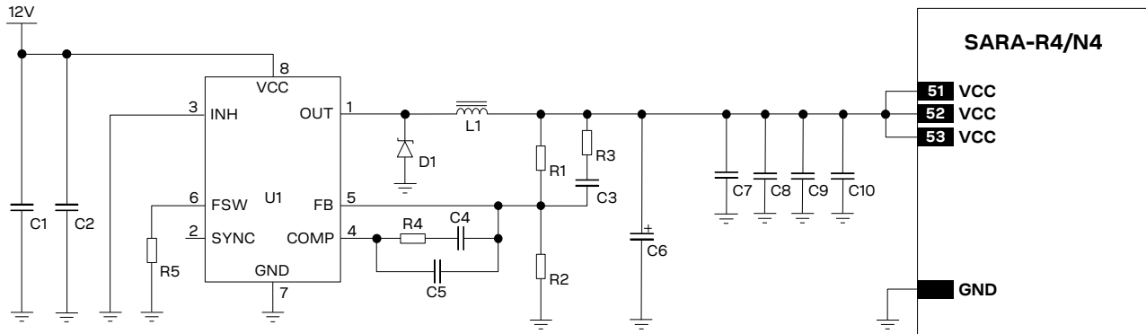
Figure 18: Example of low cost VCC supply circuit for SARA-R4 series modules, using a step-down regulator
