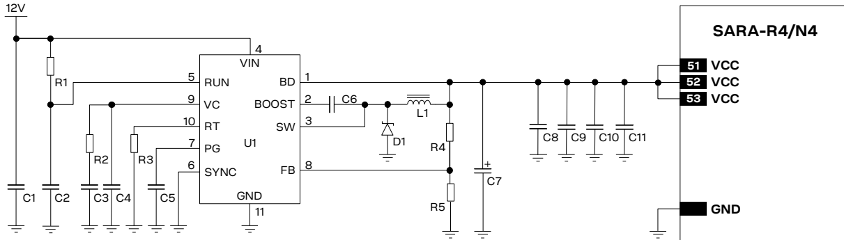
Figure 16: Example of high reliability VCC supply circuit for SARA-R4 series modules, using a step-down regulator
