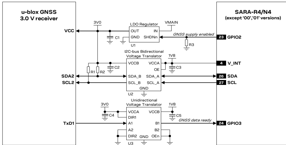
Figure 52: Application circuit for connecting SARA-R4 series modules to u-blox 3.0 V GNSS receivers
