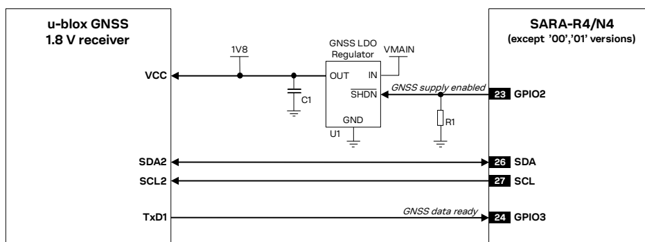
Figure 51: Application circuit for connecting SARA-R4 series modules to u-blox 1.8 V GNSS receivers
