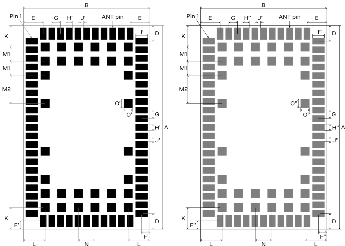
Figure 54: SARA-R4 series modules suggested footprint and paste mask (application board top view)
