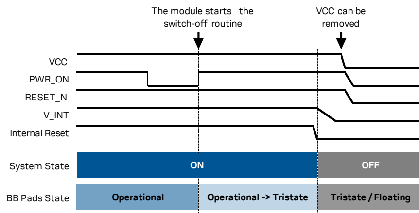
Figure 11: SARA-R4 series modules switch-off sequence by means of PWR_ON pin
