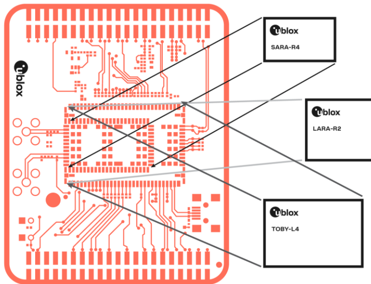
Figure 60: TOBY, SARA, LARA layout compatibility: all modules can be mounted on the same nested footprint
