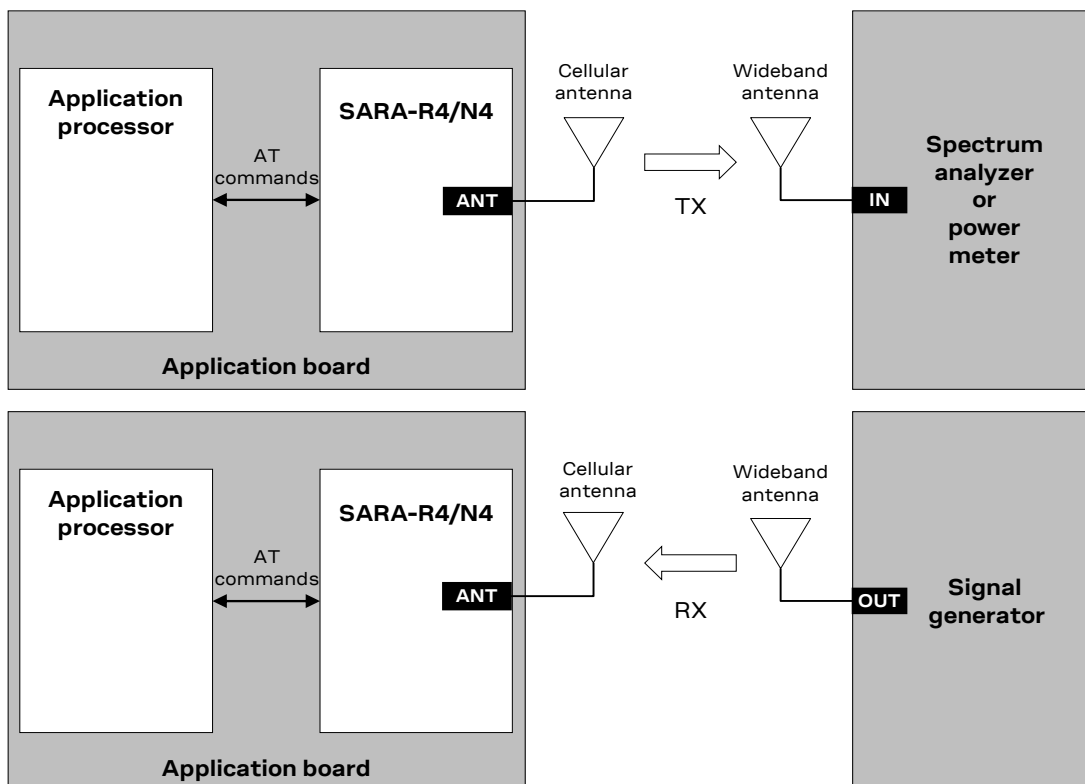
Figure 58: Setup with spectrum analyzer or power meter and signal generator for SARA-R4 series RF measurements
