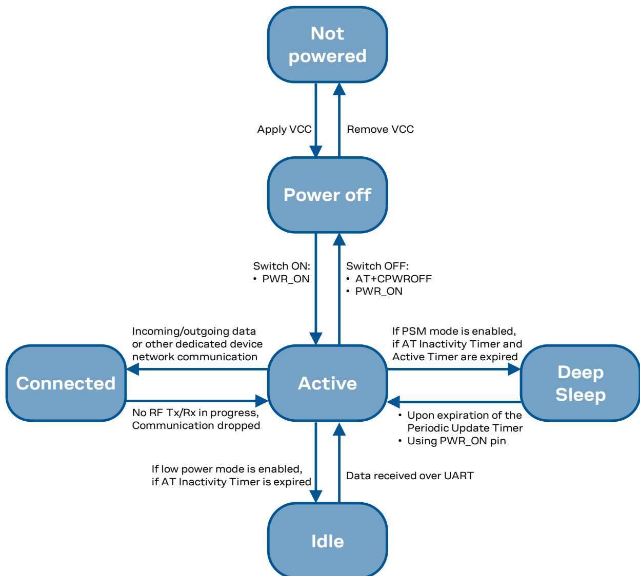
Figure 2: SARA-R4 series modules operating modes transitions
