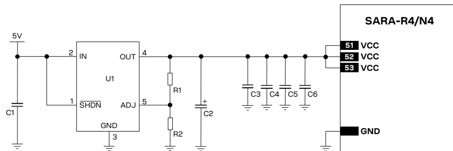
Figure 19: Example of high reliability VCC supply circuit for SARA-R4 series modules, using an LDO linear regulator
