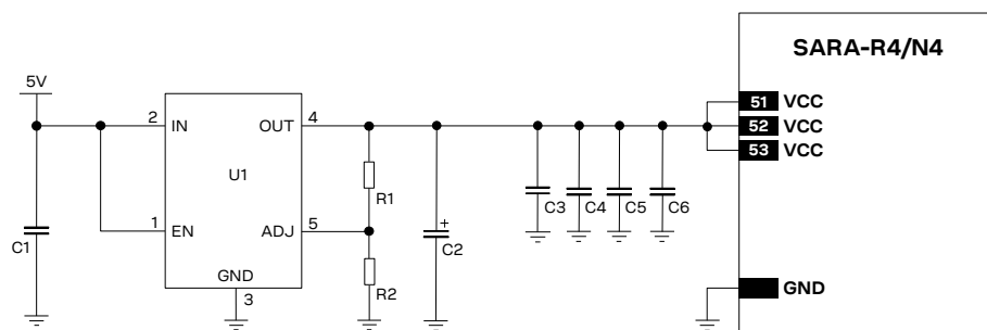
Figure 21: Example of low cost VCC supply circuit for SARA-R4 series modules, using an LDO linear regulator
