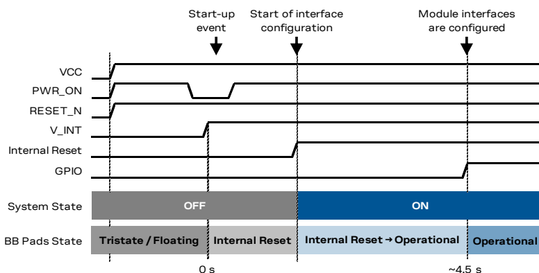
Figure 9: SARA-R4 series switch-on sequence description
