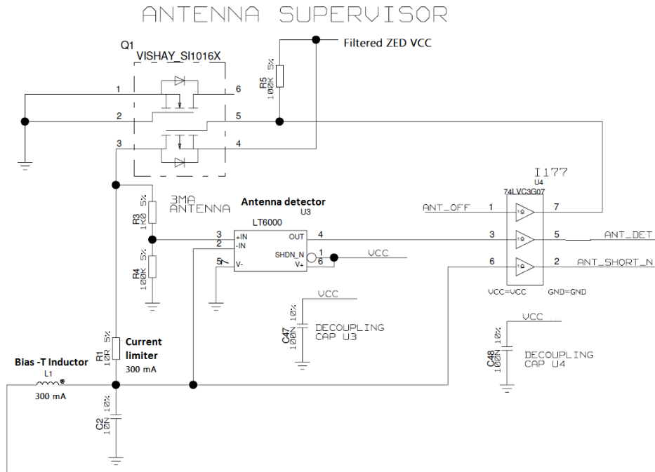
Figure 18: ZED-F9P antenna supervisor
