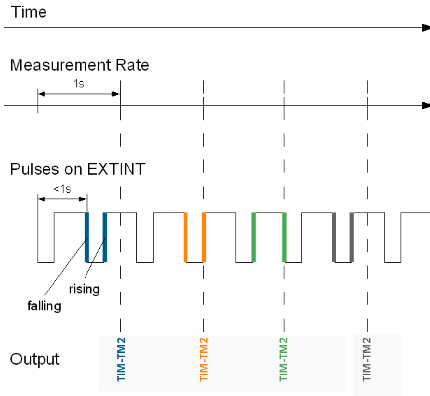
Figure 23: Timemark
