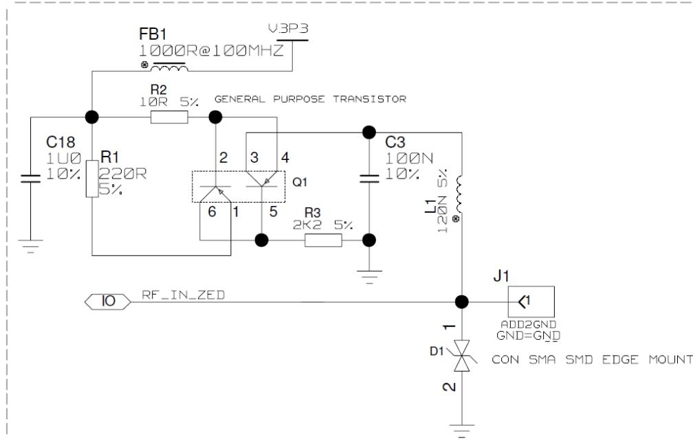
Figure 35: ZED-F9P reference design for antenna bias
