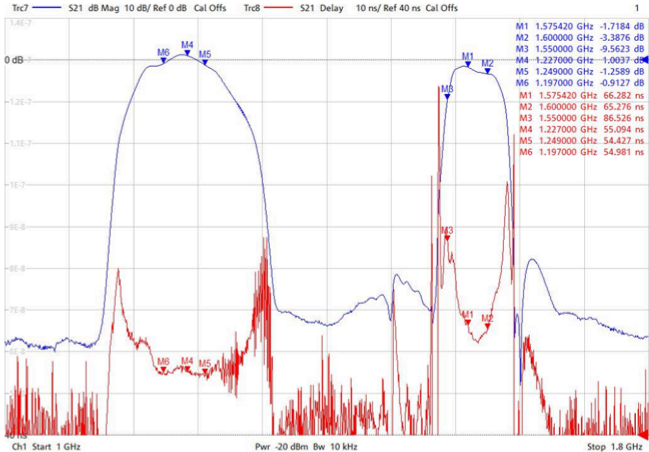
Figure 61: Low-cost L1/L2 antenna band characteristics
