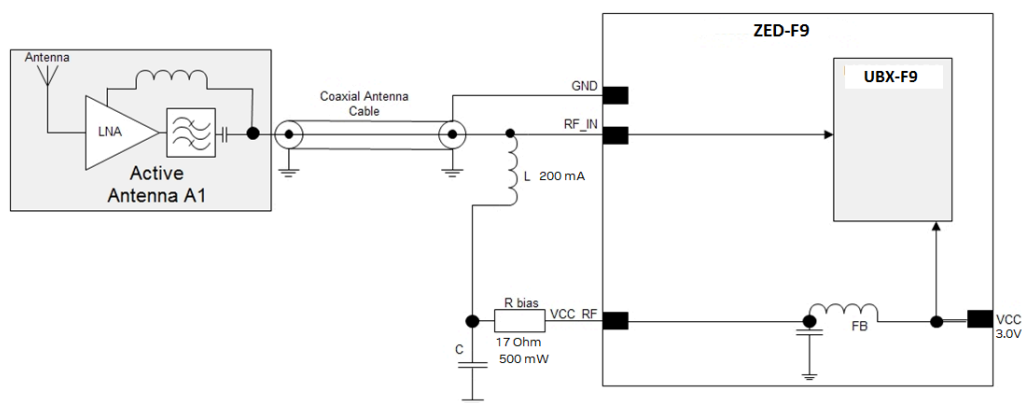
Figure 36: ZED-F9P VCC_RF antenna bias
