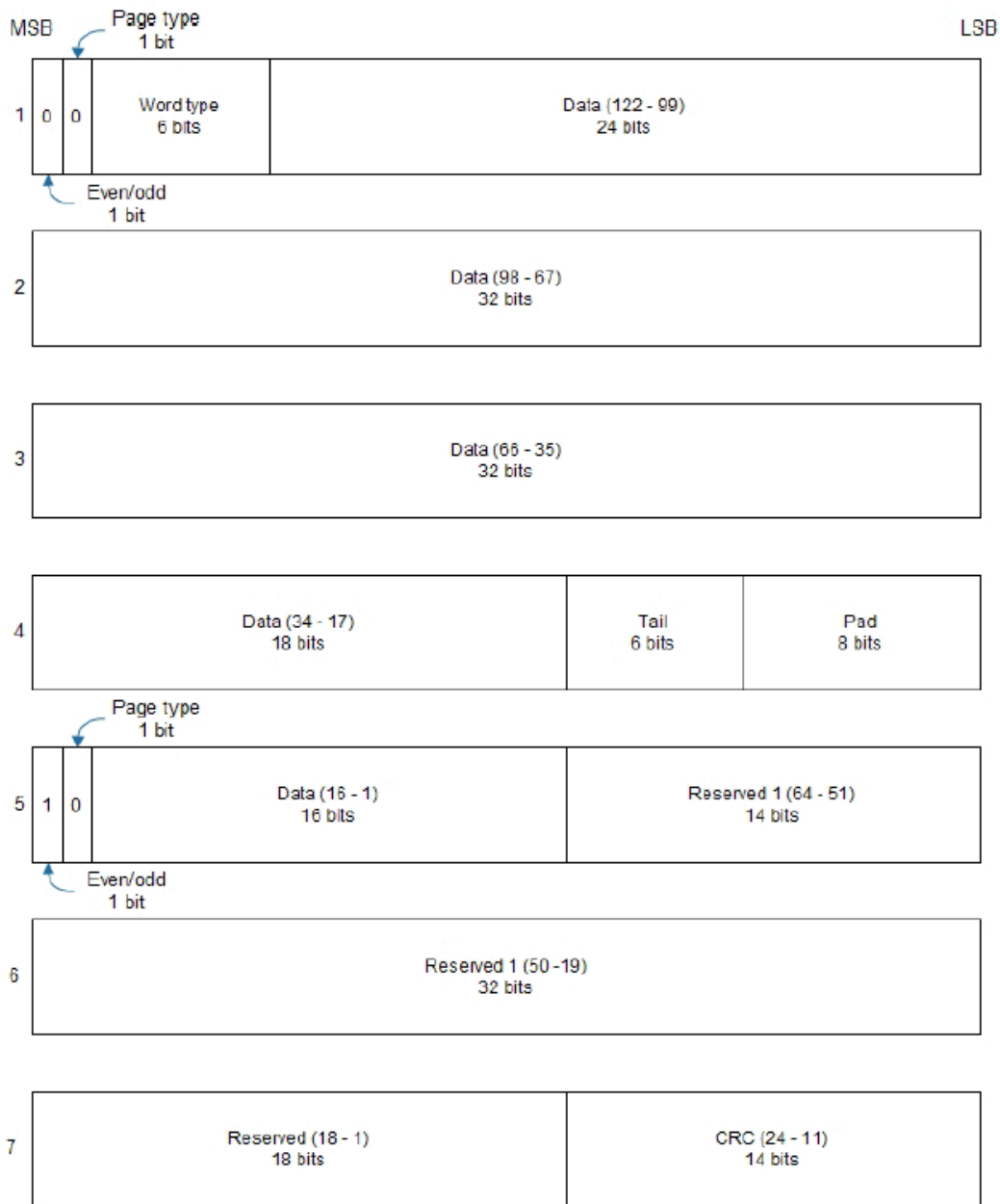
Figure 29: Galileo E5 bI/bQ subframe words
