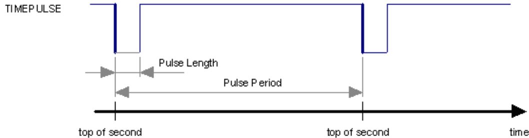
Figure 20: Time pulse
