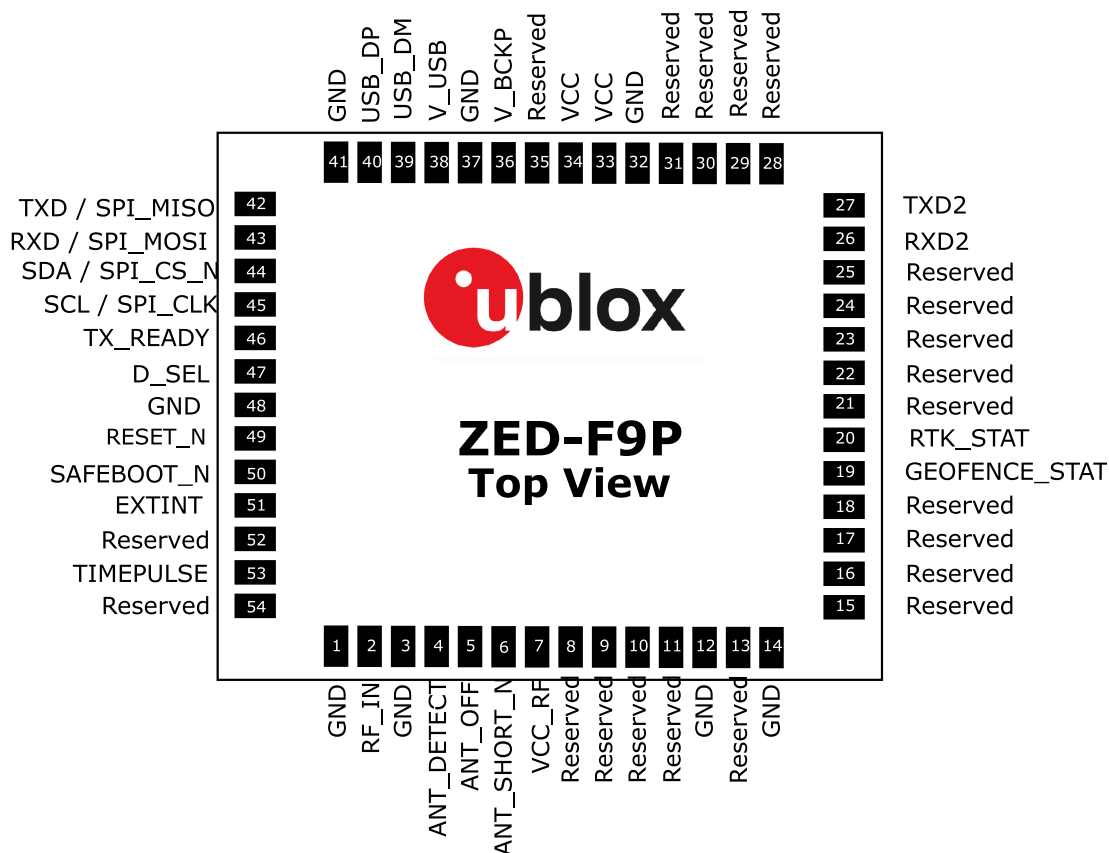
Figure 30: ZED-F9P pin assignment
