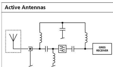
Figure 39: Active antenna EOS protection
