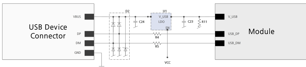
Figure 17: ZED-F9P example circuit for USB interface
