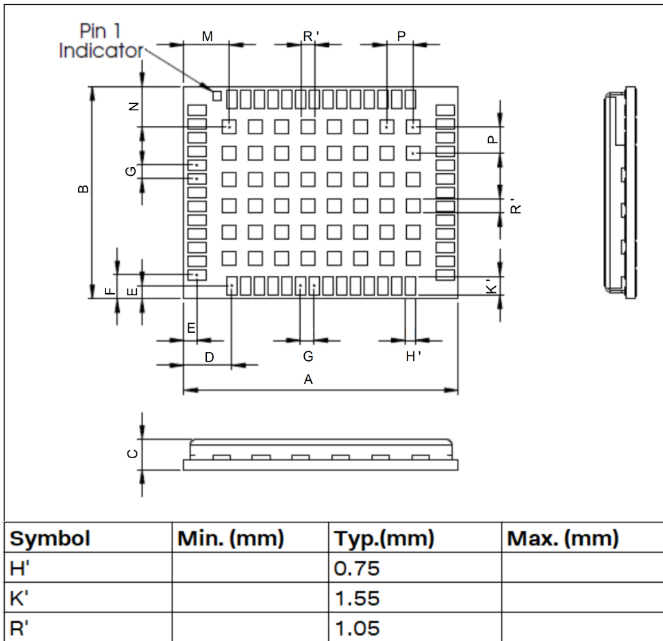
Figure 41: ZED-F9P suggested paste mask
