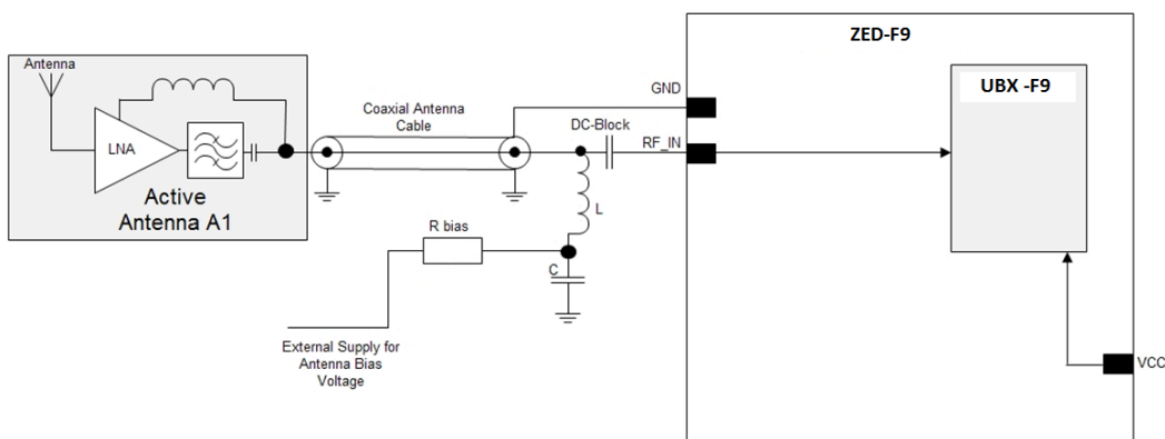
Figure 37: ZED-F9P external voltage antenna bias
