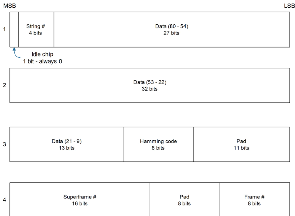
Figure 26: GLONASS subframe words
