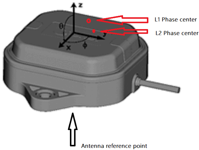
Figure 59: Stacked patch antenna
