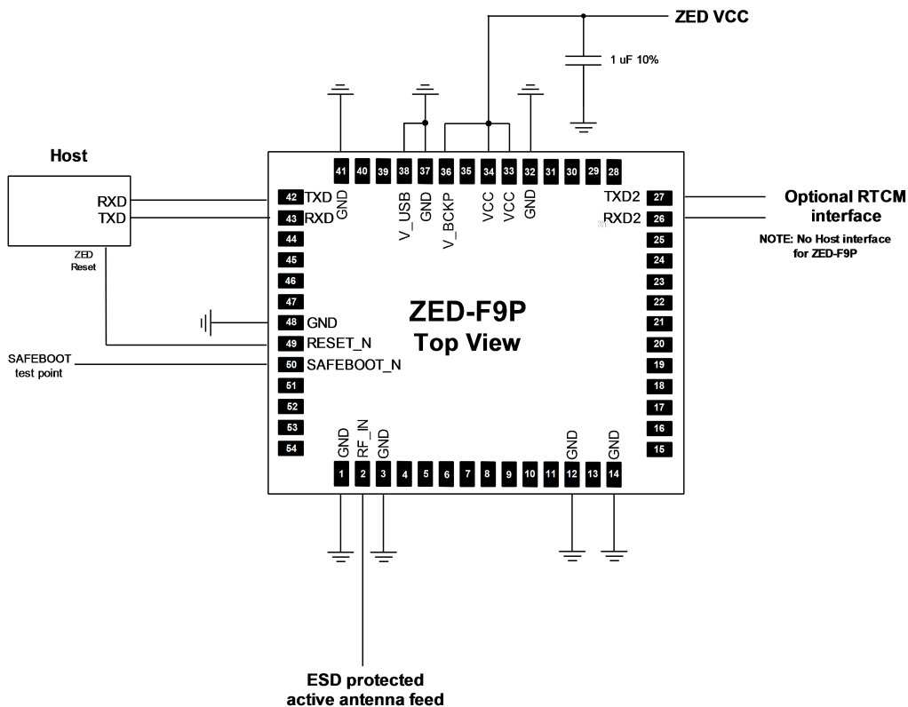
Figure 32: Minimal ZED-F9P design
