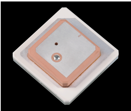
Figure 60: Ceramic stack
