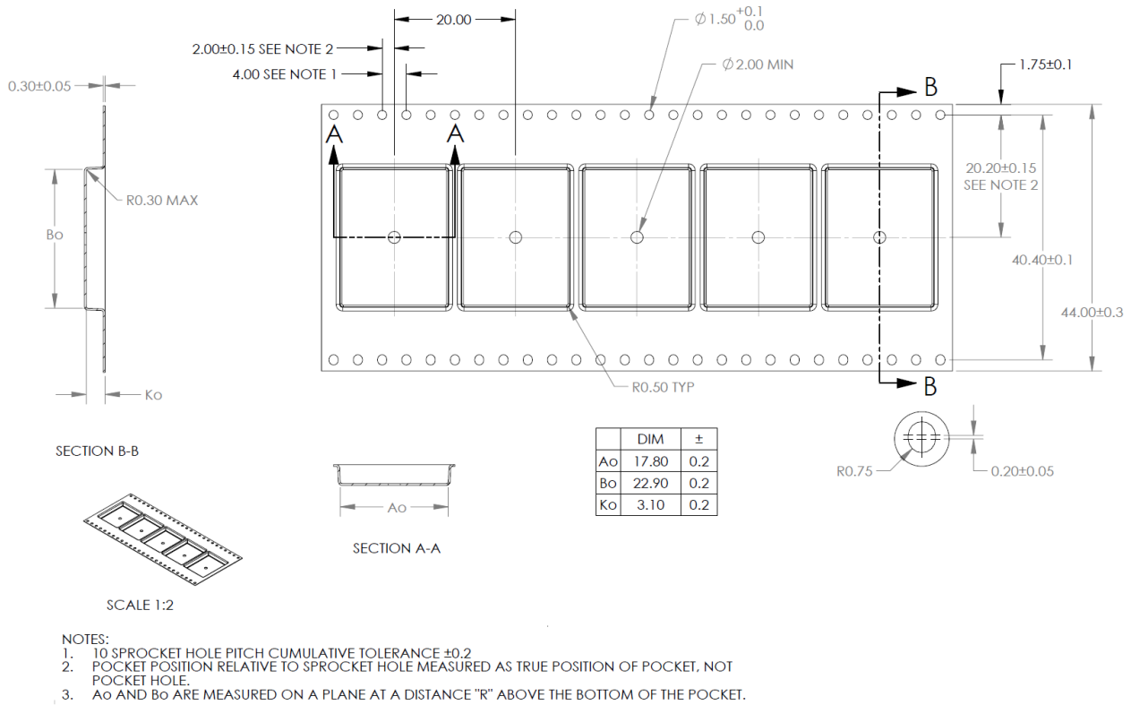
Figure 47: ZED-F9P tape dimensions (mm)
