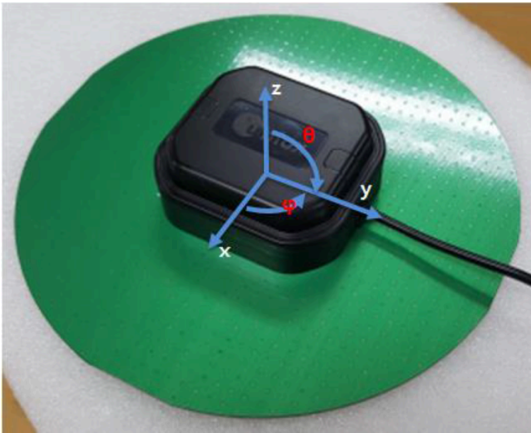
Figure 62: u-blox low-cost L1/L2 RTK antenna
