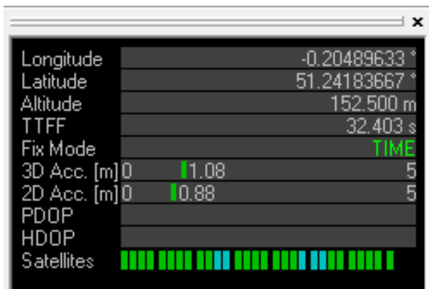
Figure 52: Base station: u-center data view in TIME mode
