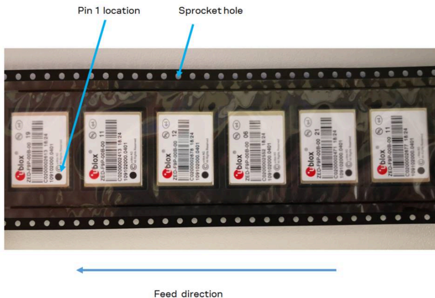
Figure 46: Orientation of ZED-F9P on the tape
