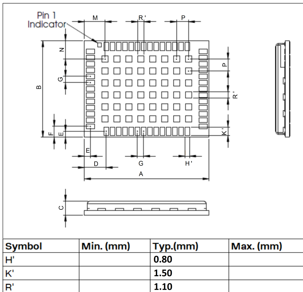
Figure 40: ZED-F9P suggested footprint (i.e. copper mask)
