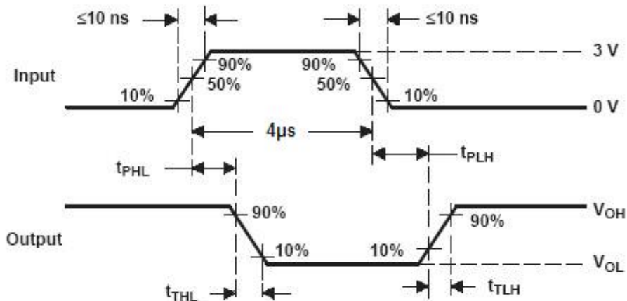
Transmitter Waveforms
